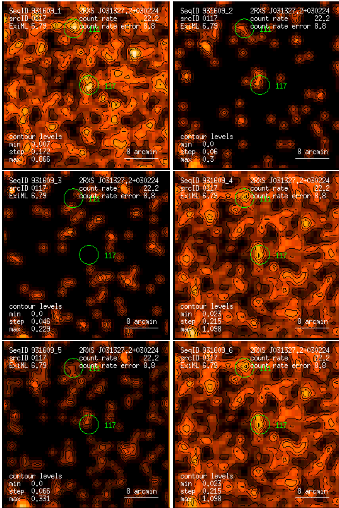
Figure 117: RASS 931609: detection 0117: band rate images, Gaussian filter: (1) PSPC channels 11 – 41, (2) 52 – 90, (3) 91 – 201, (4) 11 – 235, (5) 52 – 201, (6) 11 – 201. Broad band rates in counts/ks. Band rate contour levels in counts/ks/arcmin 2 .
