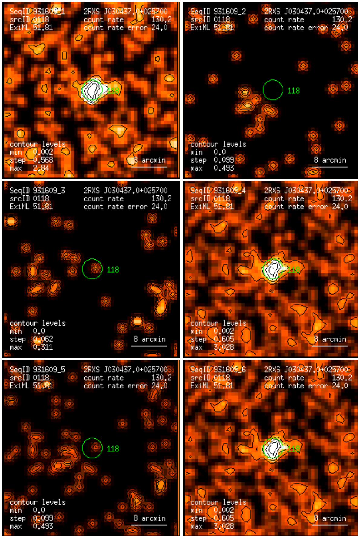
Figure 118: RASS 931609: detection 0118: band rate images, Gaussian filter: (1) PSPC channels 11 – 41, (2) 52 – 90, (3) 91 – 201, (4) 11 – 235, (5) 52 – 201, (6) 11 – 201. Broad band rates in counts/ks. Band rate contour levels in counts/ks/arcmin 2 .
