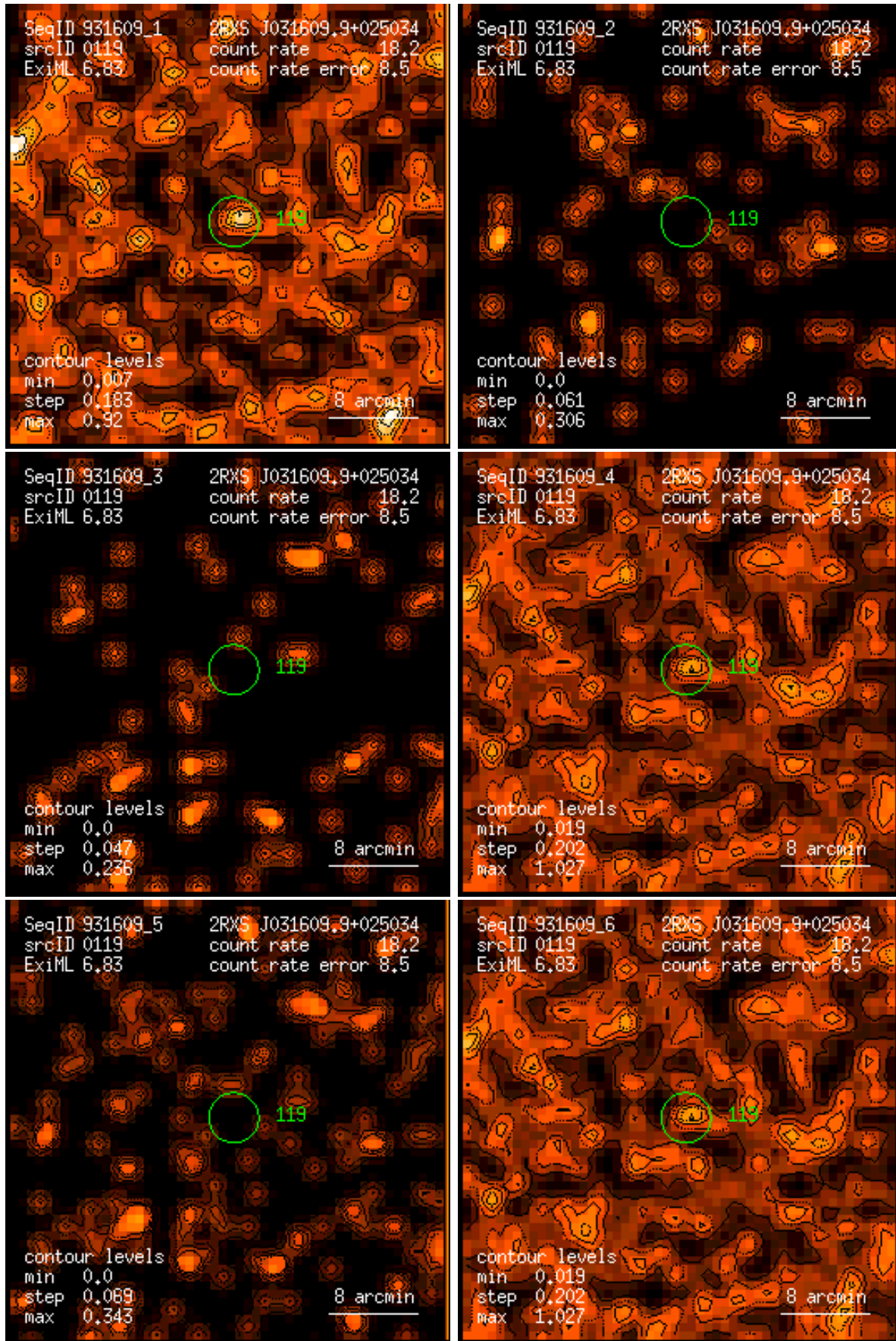
Figure 119: RASS 931609: detection 0119: band rate images, Gaussian filter: (1) PSPC channels 11 – 41, (2) 52 – 90, (3) 91 – 201, (4) 11 – 235, (5) 52 – 201, (6) 11 – 201. Broad band rates in counts/ks. Band rate contour levels in counts/ks/arcmin 2 .
