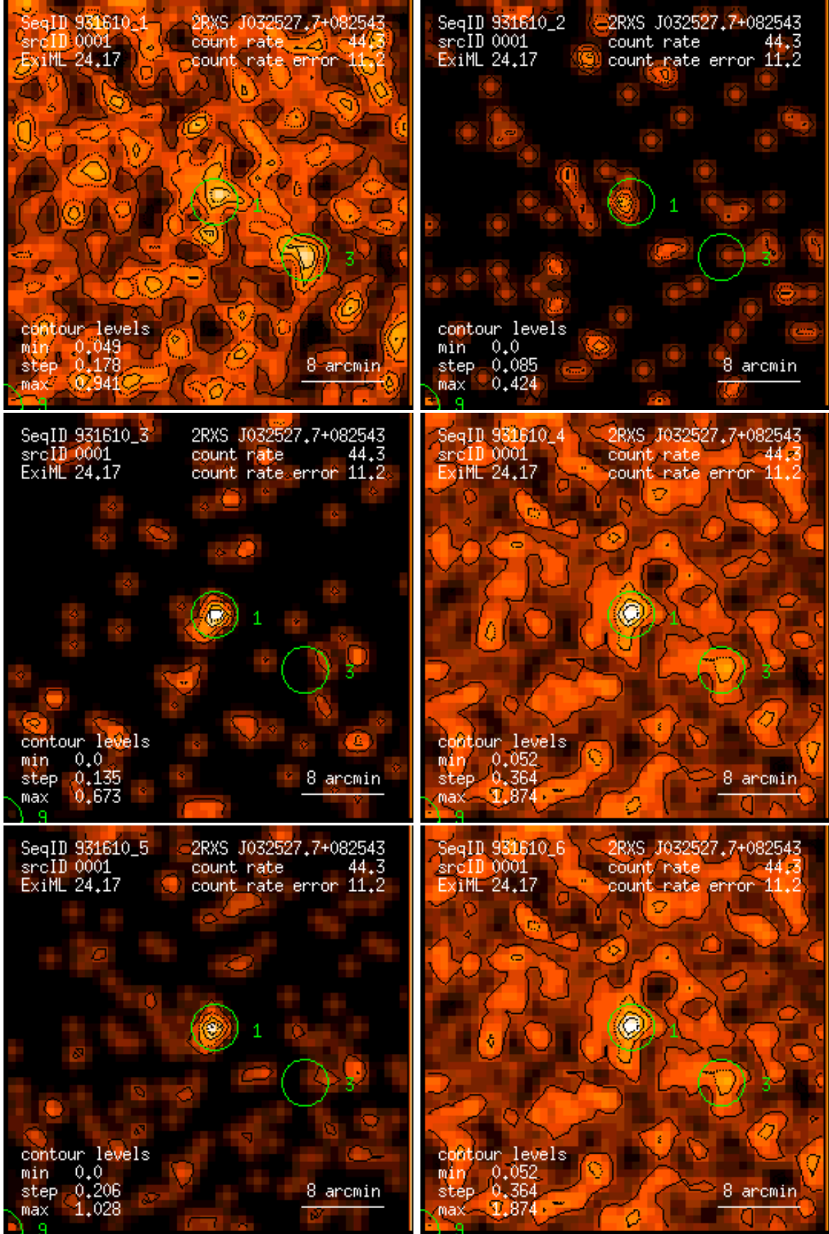
Figure 1: RASS 931610: detection 0001: band rate images, Gaussian filter: (1) PSPC channels 11 – 41, (2) 52 – 90, (3) 91 – 201, (4) 11 – 235, (5) 52 – 201, (6) 11 – 201. Broad band rates in counts/ks. Band rate contour levels in counts/ks/arcmin 2 .
