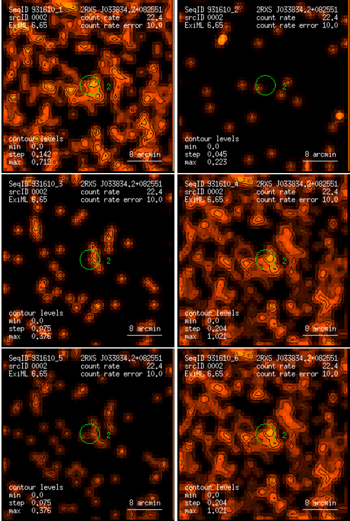
Figure 2: RASS 931610: detection 0002: band rate images, Gaussian filter: (1) PSPC channels 11 – 41, (2) 52 – 90, (3) 91 – 201, (4) 11 – 235, (5) 52 – 201, (6) 11 – 201. Broad band rates in counts/ks. Band rate contour levels in counts/ks/arcmin 2 .
