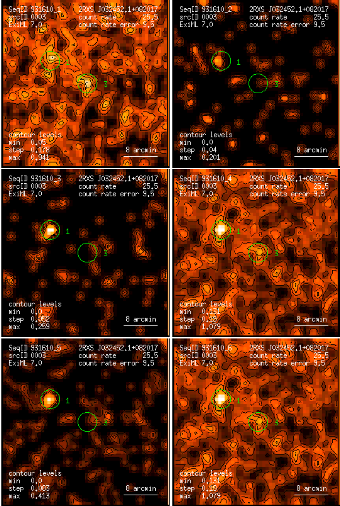
Figure 3: RASS 931610: detection 0003: band rate images, Gaussian filter: (1) PSPC channels 11 – 41, (2) 52 – 90, (3) 91 – 201, (4) 11 – 235, (5) 52 – 201, (6) 11 – 201. Broad band rates in counts/ks. Band rate contour levels in counts/ks/arcmin 2 .
