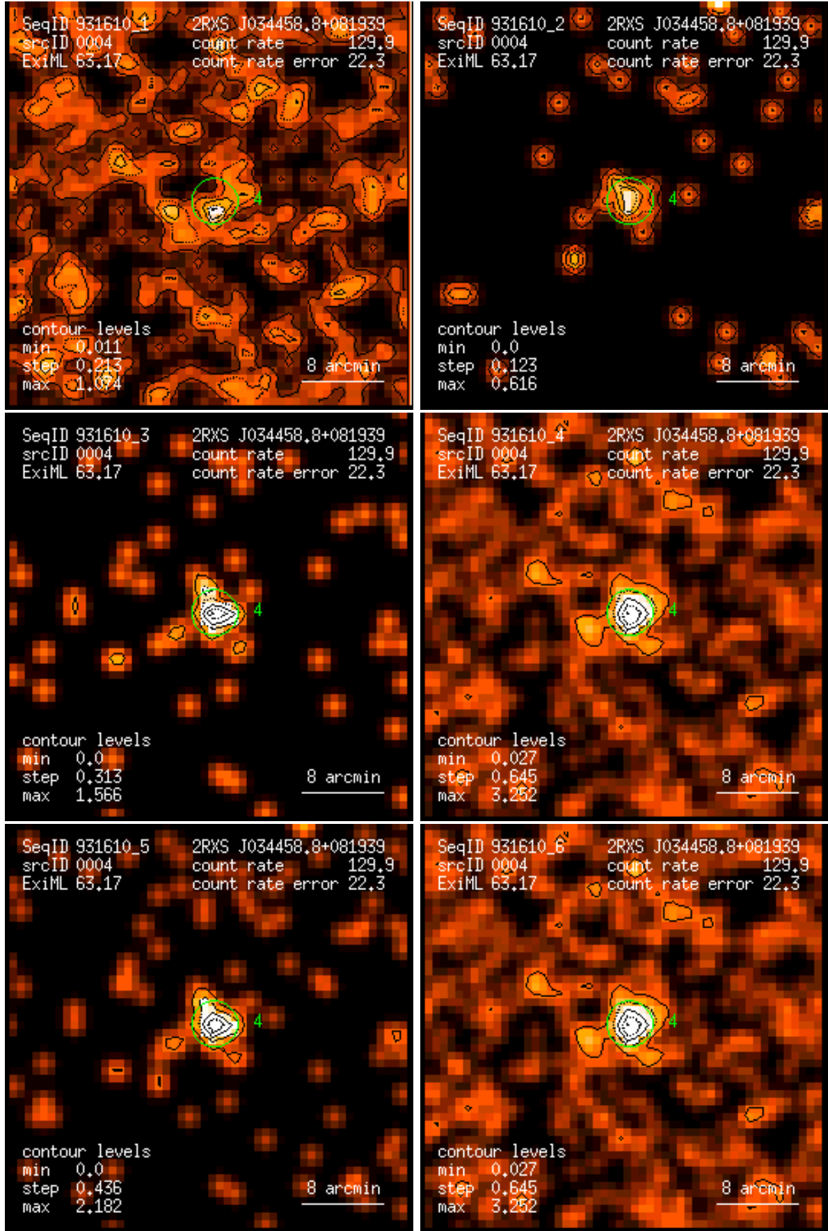
Figure 4: RASS 931610: detection 0004: band rate images, Gaussian filter: (1) PSPC channels 11 – 41, (2) 52 – 90, (3) 91 – 201, (4) 11 – 235, (5) 52 – 201, (6) 11 – 201. Broad band rates in counts/ks. Band rate contour levels in counts/ks/arcmin 2 .
