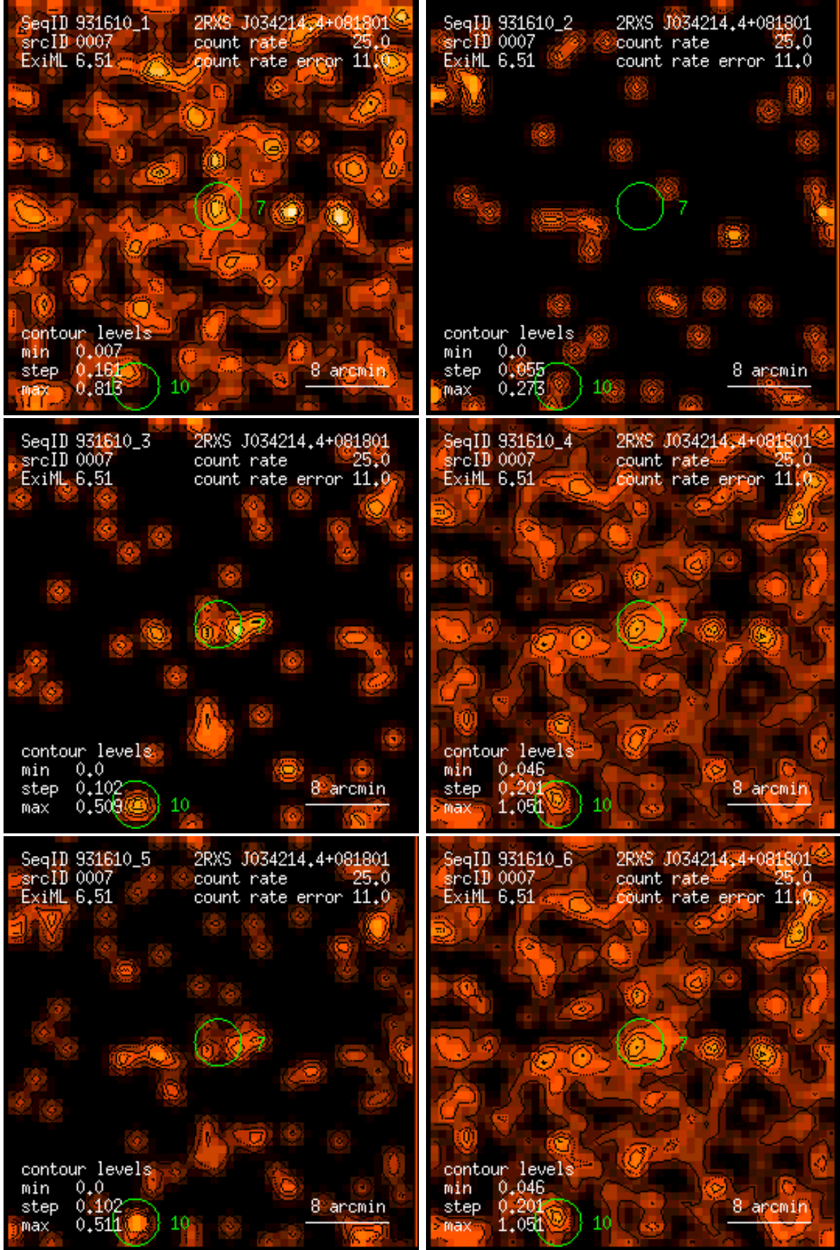
Figure 7: RASS 931610: detection 0007: band rate images, Gaussian filter: (1) PSPC channels 11 – 41, (2) 52 – 90, (3) 91 – 201, (4) 11 – 235, (5) 52 – 201, (6) 11 – 201. Broad band rates in counts/ks. Band rate contour levels in counts/ks/arcmin 2 .
