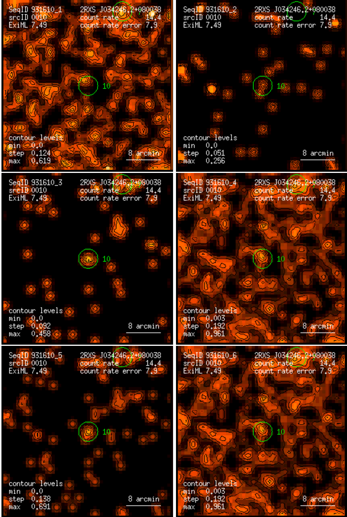
Figure 10: RASS 931610: detection 0010: band rate images, Gaussian filter: (1) PSPC channels 11 – 41, (2) 52 – 90, (3) 91 – 201, (4) 11 – 235, (5) 52 – 201, (6) 11 – 201. Broad band rates in counts/ks. Band rate contour levels in counts/ks/arcmin 2 .
