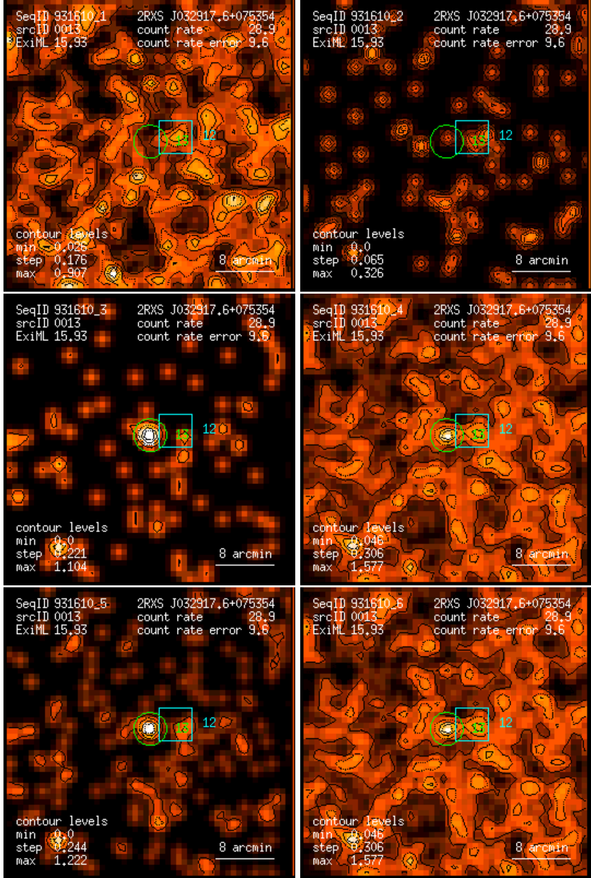
Figure 13: RASS 931610: detection 0013: band rate images, Gaussian filter: (1) PSPC channels 11 – 41, (2) 52 – 90, (3) 91 – 201, (4) 11 – 235, (5) 52 – 201, (6) 11 – 201. Broad band rates in counts/ks. Band rate contour levels in counts/ks/arcmin 2 .
