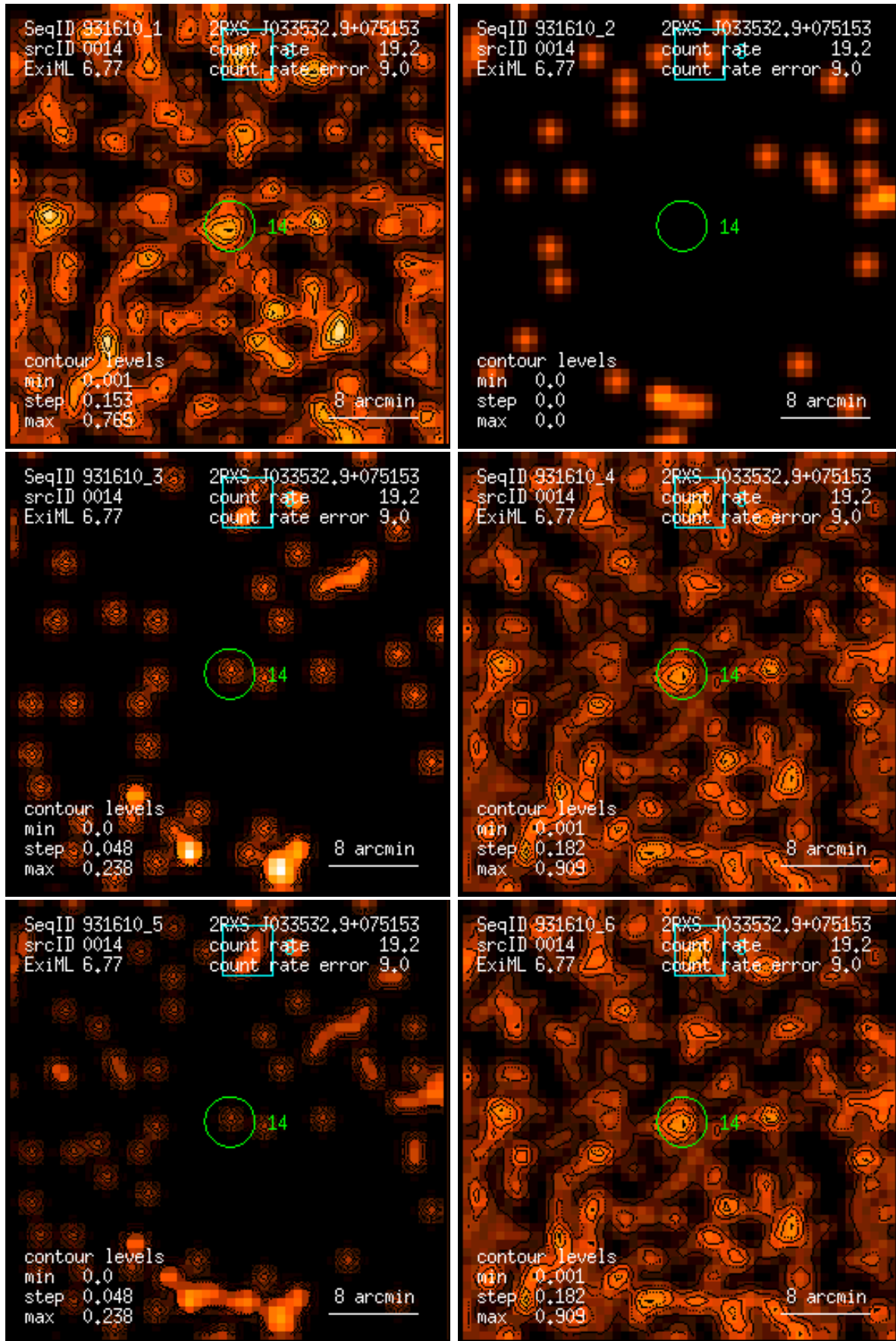
Figure 14: RASS 931610: detection 0014: band rate images, Gaussian filter: (1) PSPC channels 11 – 41, (2) 52 – 90, (3) 91 – 201, (4) 11 – 235, (5) 52 – 201, (6) 11 – 201. Broad band rates in counts/ks. Band rate contour levels in counts/ks/arcmin 2 .
