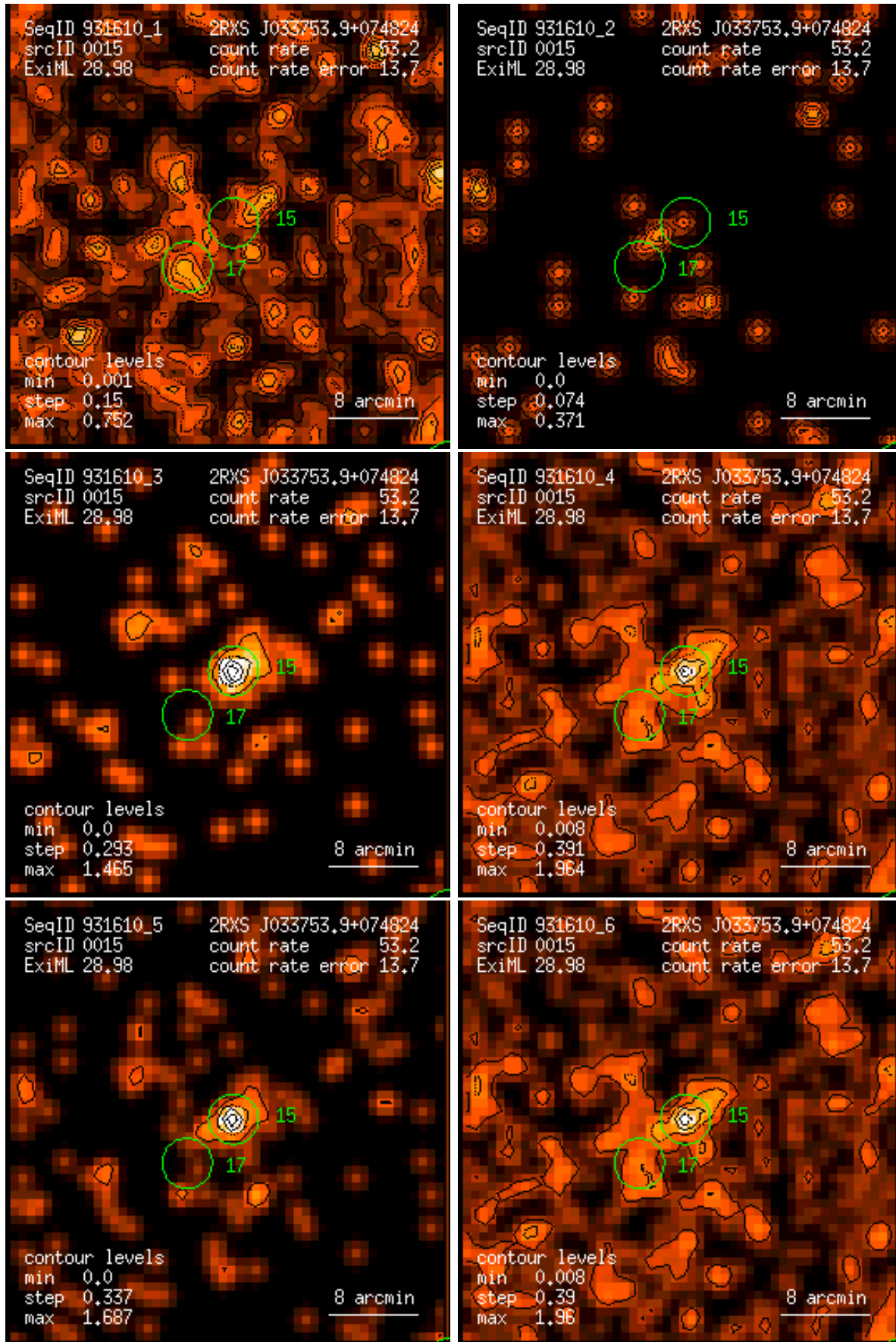
Figure 15: RASS 931610: detection 0015: band rate images, Gaussian filter: (1) PSPC channels 11 – 41, (2) 52 – 90, (3) 91 – 201, (4) 11 – 235, (5) 52 – 201, (6) 11 – 201. Broad band rates in counts/ks. Band rate contour levels in counts/ks/arcmin 2 .
