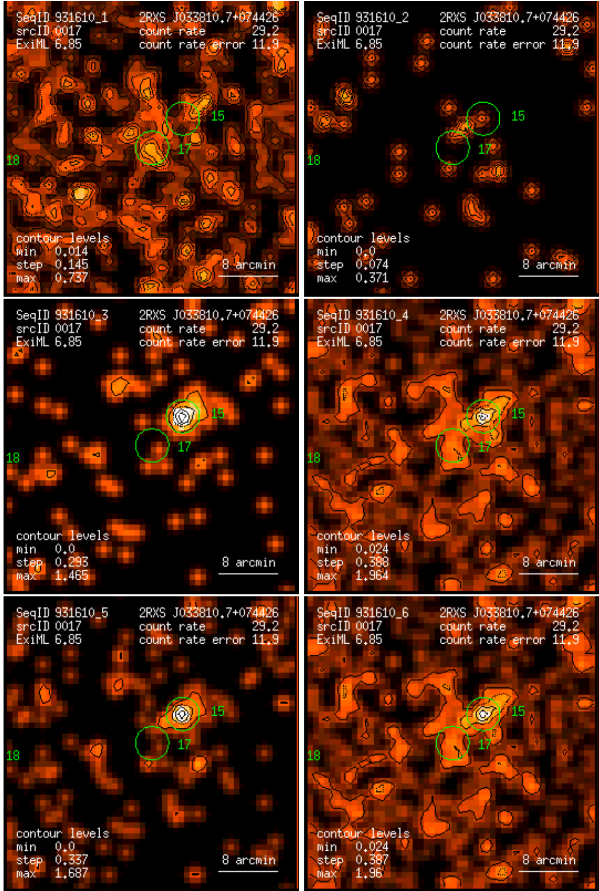
Figure 17: RASS 931610: detection 0017: band rate images, Gaussian filter: (1) PSPC channels 11 – 41, (2) 52 – 90, (3) 91 – 201, (4) 11 – 235, (5) 52 – 201, (6) 11 – 201. Broad band rates in counts/ks. Band rate contour levels in counts/ks/arcmin 2 .
