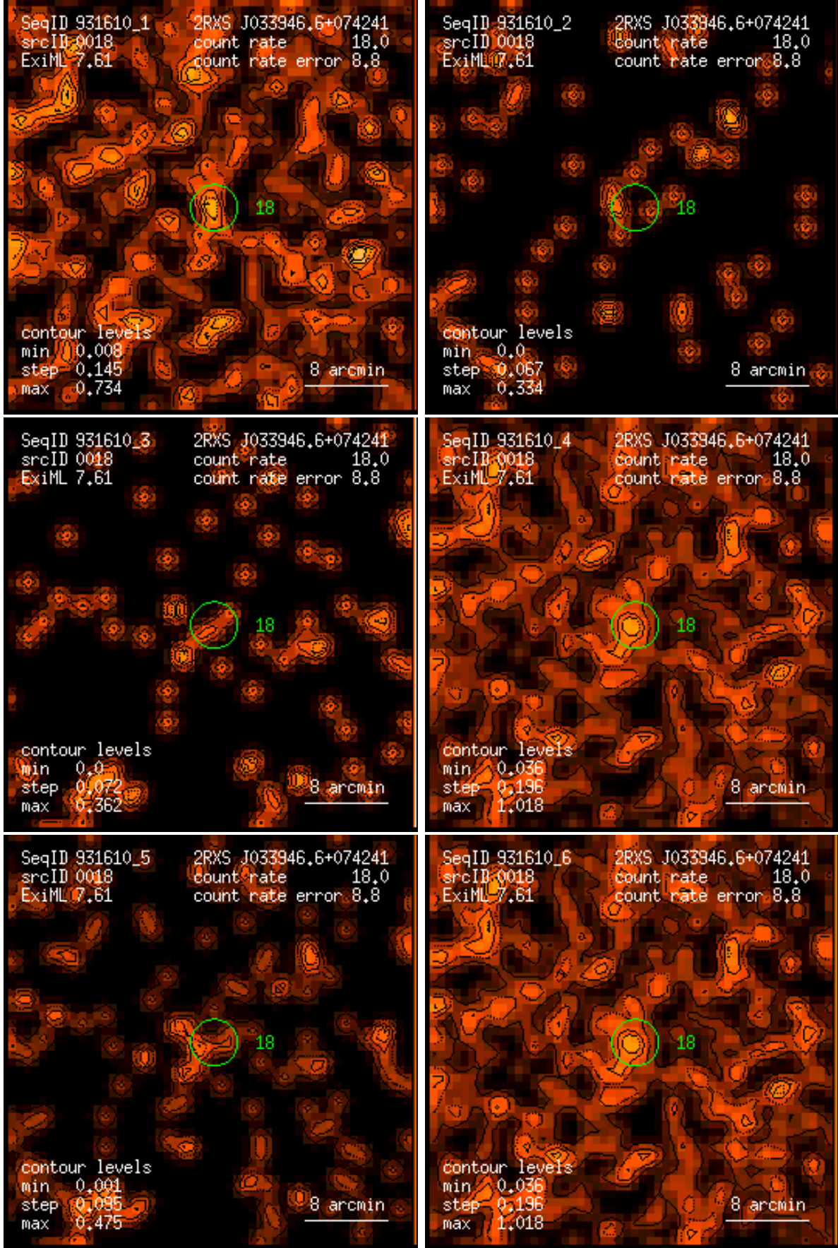
Figure 18: RASS 931610: detection 0018: band rate images, Gaussian filter: (1) PSPC channels 11 – 41, (2) 52 – 90, (3) 91 – 201, (4) 11 – 235, (5) 52 – 201, (6) 11 – 201. Broad band rates in counts/ks. Band rate contour levels in counts/ks/arcmin 2 .
