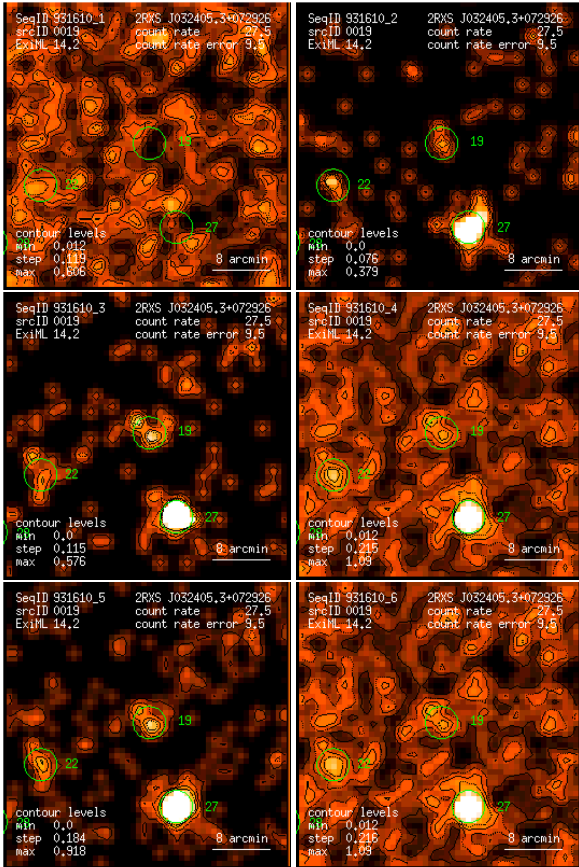
Figure 19: RASS 931610: detection 0019: band rate images, Gaussian filter: (1) PSPC channels 11 – 41, (2) 52 – 90, (3) 91 – 201, (4) 11 – 235, (5) 52 – 201, (6) 11 – 201. Broad band rates in counts/ks. Band rate contour levels in counts/ks/arcmin 2 .
