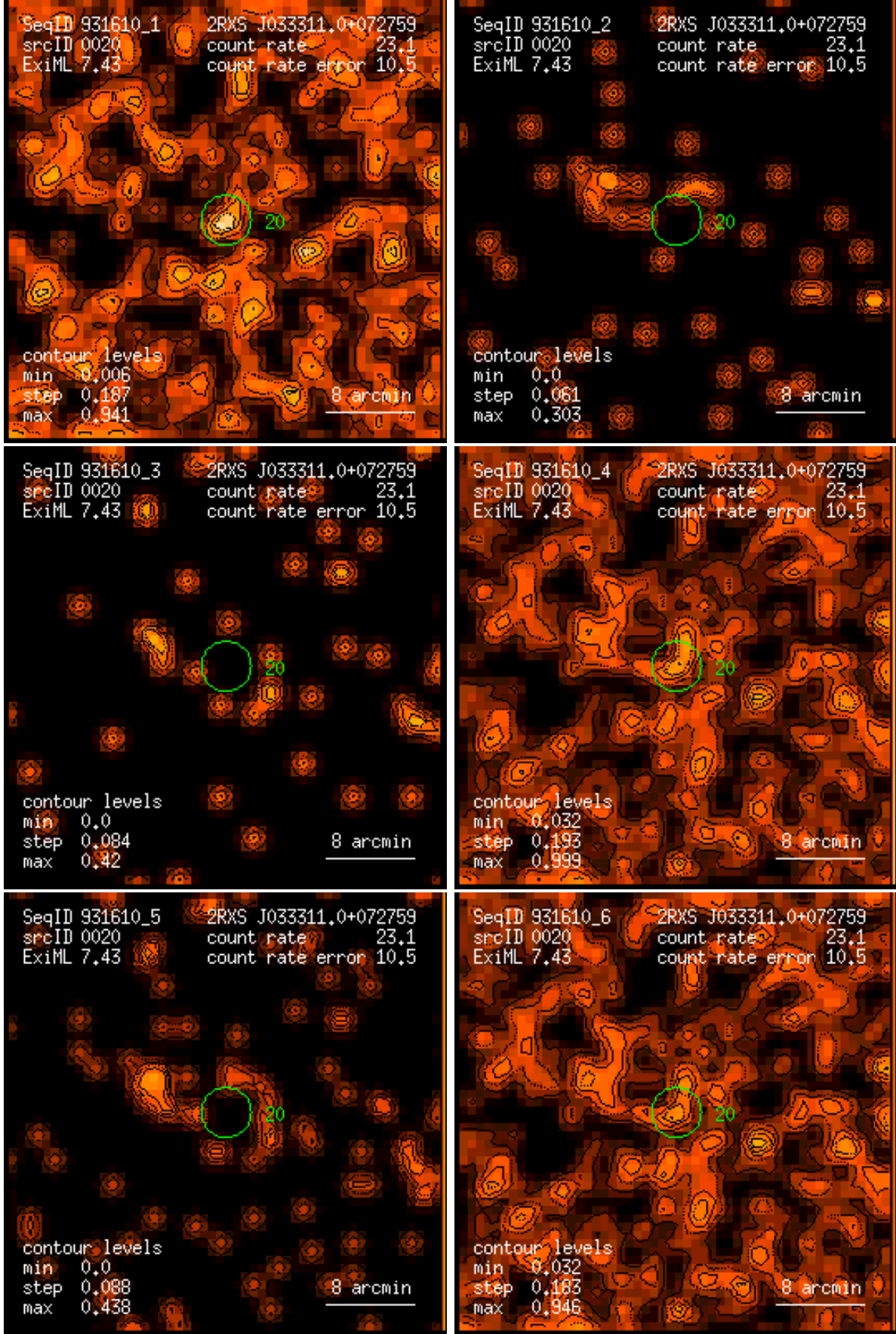
Figure 20: RASS 931610: detection 0020: band rate images, Gaussian filter: (1) PSPC channels 11 – 41, (2) 52 – 90, (3) 91 – 201, (4) 11 – 235, (5) 52 – 201, (6) 11 – 201. Broad band rates in counts/ks. Band rate contour levels in counts/ks/arcmin 2 .
