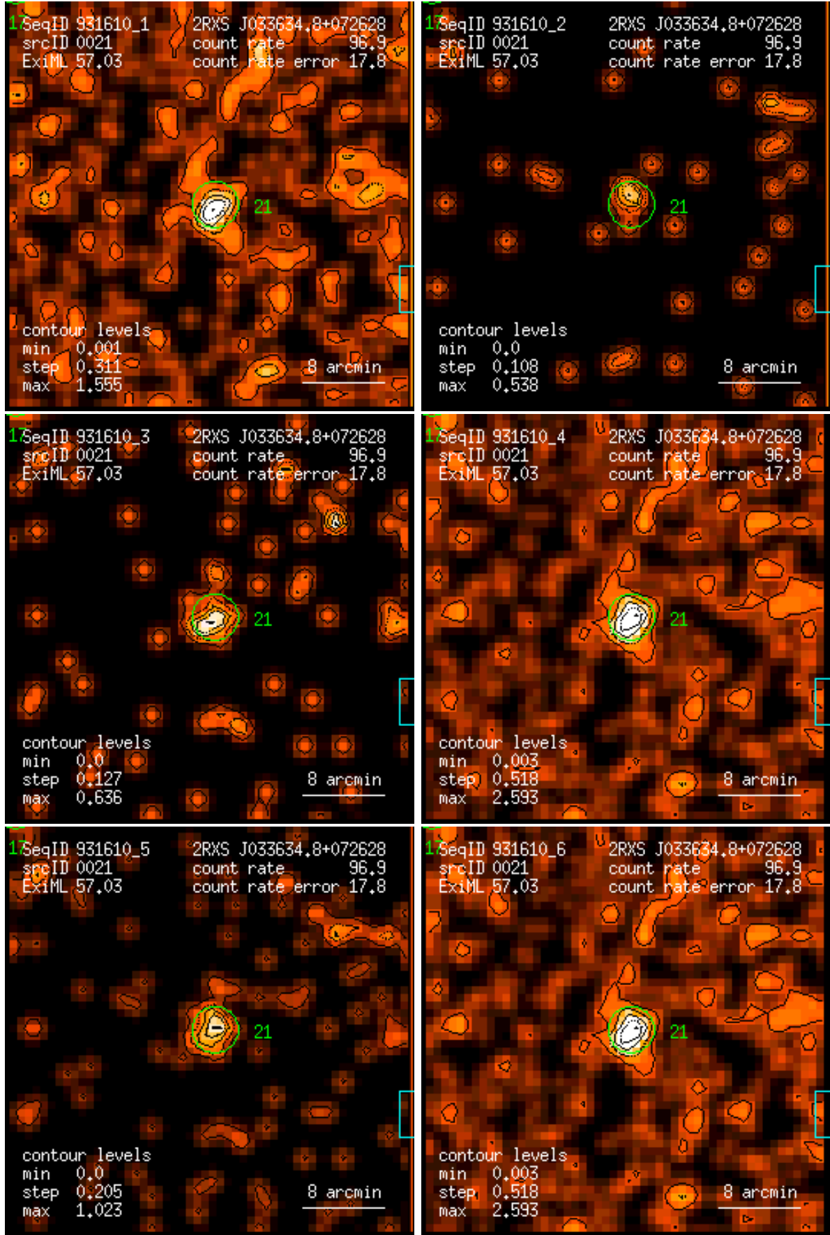
Figure 21: RASS 931610: detection 0021: band rate images, Gaussian filter: (1) PSPC channels 11 – 41, (2) 52 – 90, (3) 91 – 201, (4) 11 – 235, (5) 52 – 201, (6) 11 – 201. Broad band rates in counts/ks. Band rate contour levels in counts/ks/arcmin 2 .
