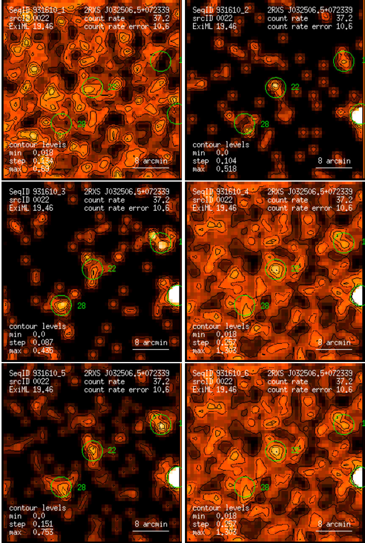
Figure 22: RASS 931610: detection 0022: band rate images, Gaussian filter: (1) PSPC channels 11 – 41, (2) 52 – 90, (3) 91 – 201, (4) 11 – 235, (5) 52 – 201, (6) 11 – 201. Broad band rates in counts/ks. Band rate contour levels in counts/ks/arcmin 2 .
