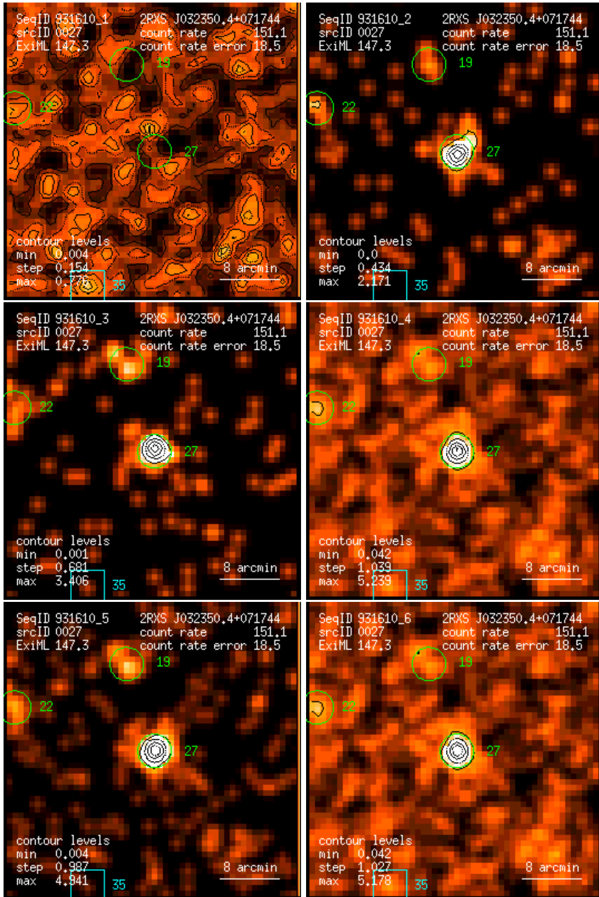
Figure 27: RASS 931610: detection 0027: band rate images, Gaussian filter: (1) PSPC channels 11 – 41, (2) 52 – 90, (3) 91 – 201, (4) 11 – 235, (5) 52 – 201, (6) 11 – 201. Broad band rates in counts/ks. Band rate contour levels in counts/ks/arcmin 2 .
