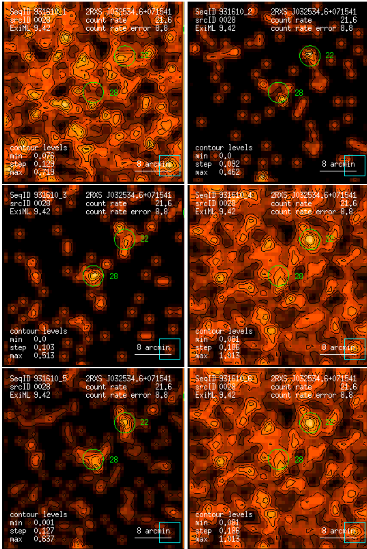
Figure 28: RASS 931610: detection 0028: band rate images, Gaussian filter: (1) PSPC channels 11 – 41, (2) 52 – 90, (3) 91 – 201, (4) 11 – 235, (5) 52 – 201, (6) 11 – 201. Broad band rates in counts/ks. Band rate contour levels in counts/ks/arcmin 2 .
