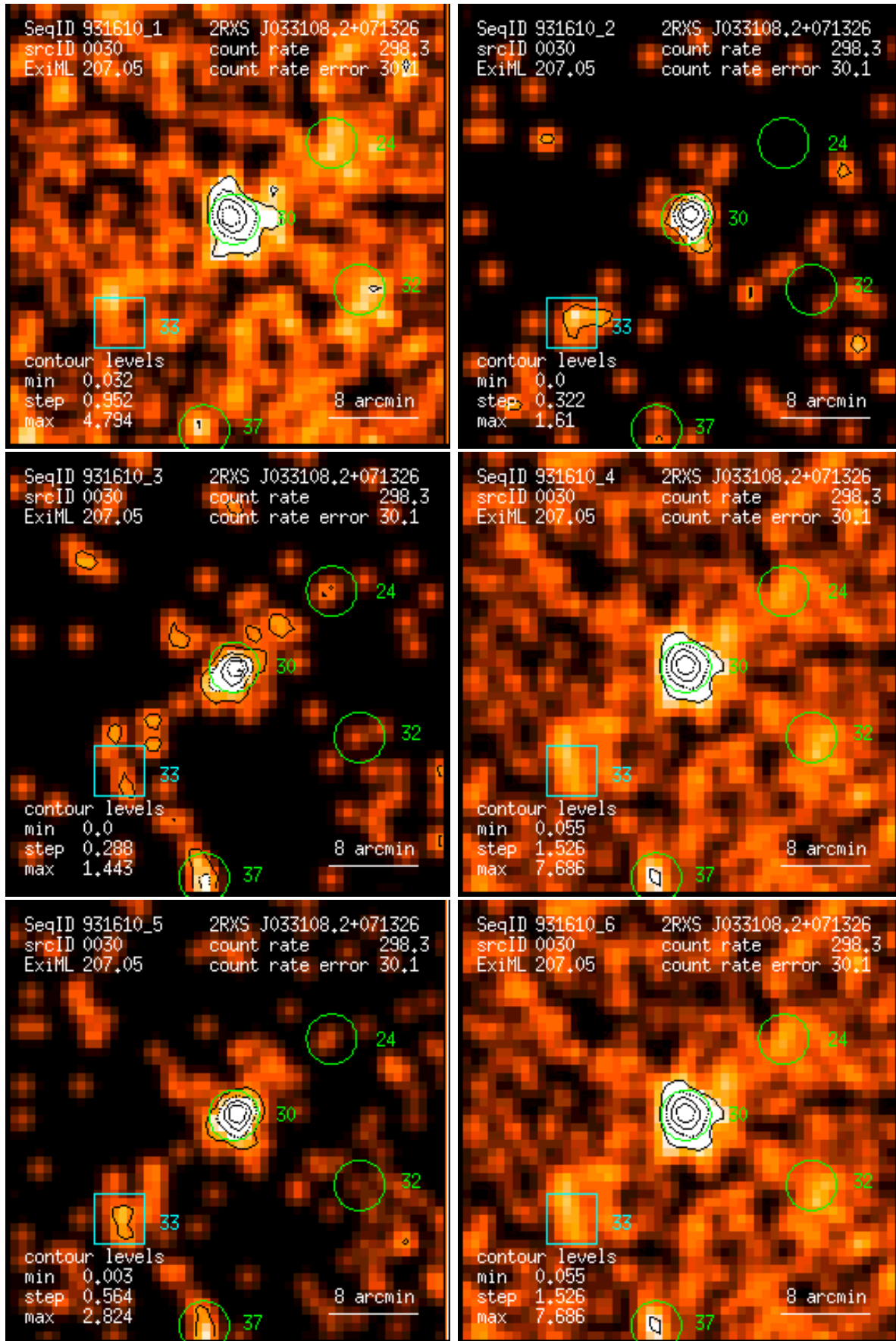
Figure 30: RASS 931610: detection 0030: band rate images, Gaussian filter: (1) PSPC channels 11 – 41, (2) 52 – 90, (3) 91 – 201, (4) 11 – 235, (5) 52 – 201, (6) 11 – 201. Broad band rates in counts/ks. Band rate contour levels in counts/ks/arcmin 2 .
