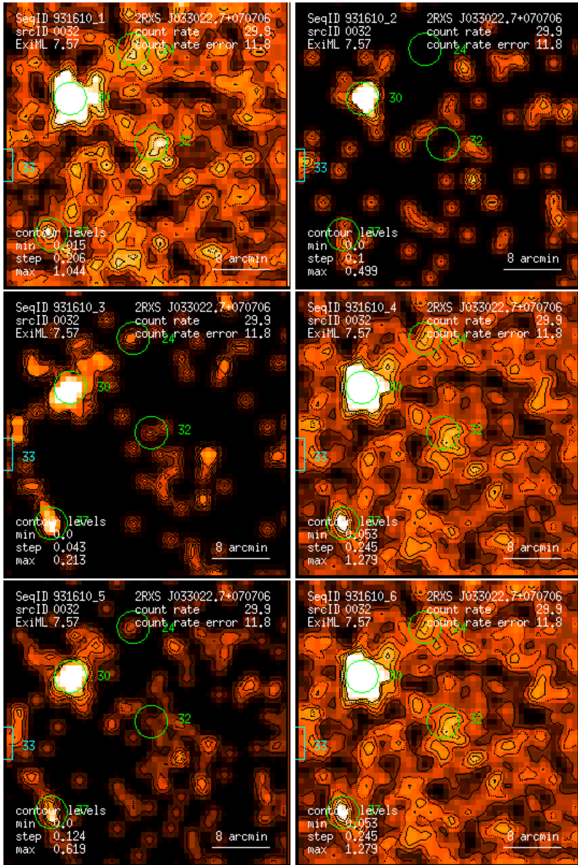
Figure 32: RASS 931610: detection 0032: band rate images, Gaussian filter: (1) PSPC channels 11 – 41, (2) 52 – 90, (3) 91 – 201, (4) 11 – 235, (5) 52 – 201, (6) 11 – 201. Broad band rates in counts/ks. Band rate contour levels in counts/ks/arcmin 2 .
