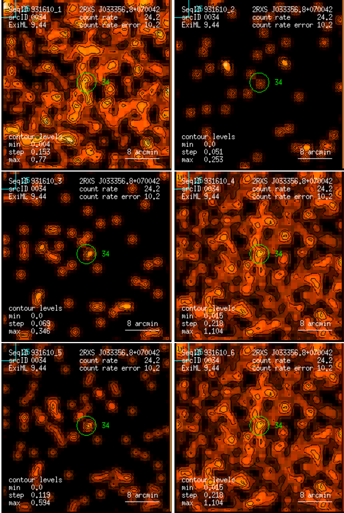
Figure 34: RASS 931610: detection 0034: band rate images, Gaussian filter: (1) PSPC channels 11 – 41, (2) 52 – 90, (3) 91 – 201, (4) 11 – 235, (5) 52 – 201, (6) 11 – 201. Broad band rates in counts/ks. Band rate contour levels in counts/ks/arcmin 2 .
