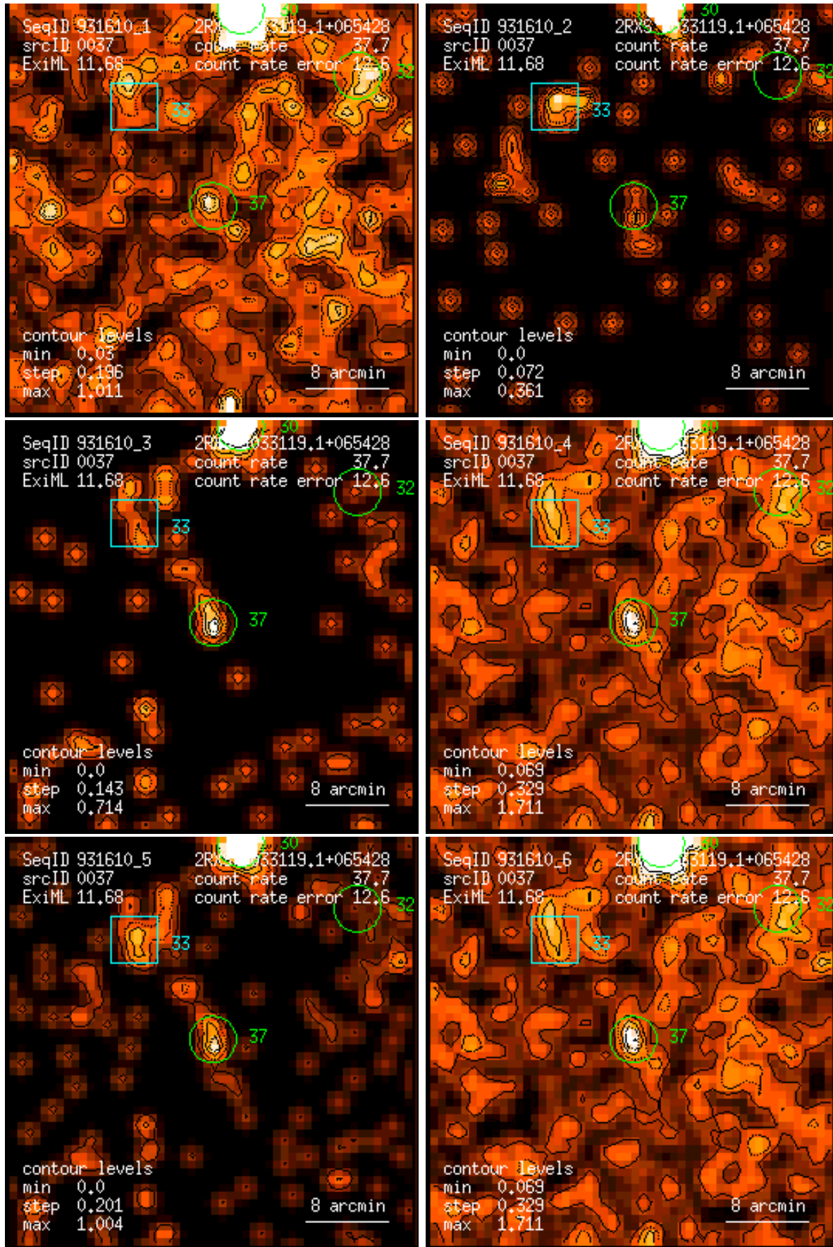
Figure 37: RASS 931610: detection 0037: band rate images, Gaussian filter: (1) PSPC channels 11 – 41, (2) 52 – 90, (3) 91 – 201, (4) 11 – 235, (5) 52 – 201, (6) 11 – 201. Broad band rates in counts/ks. Band rate contour levels in counts/ks/arcmin 2 .
