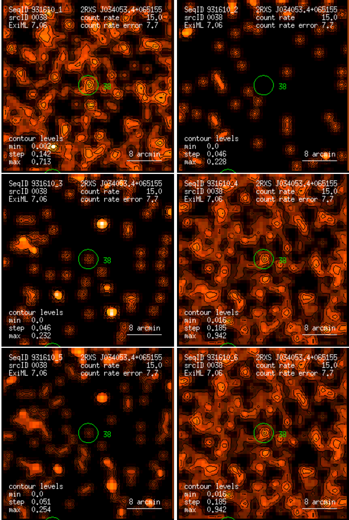
Figure 38: RASS 931610: detection 0038: band rate images, Gaussian filter: (1) PSPC channels 11 – 41, (2) 52 – 90, (3) 91 – 201, (4) 11 – 235, (5) 52 – 201, (6) 11 – 201. Broad band rates in counts/ks. Band rate contour levels in counts/ks/arcmin 2 .
