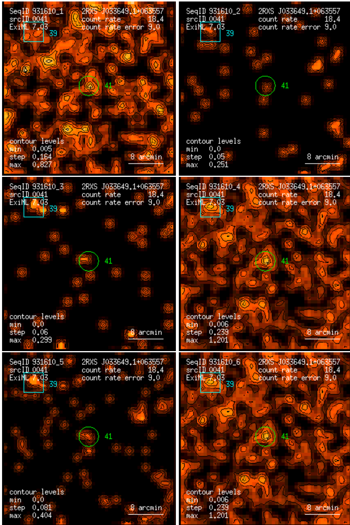
Figure 41: RASS 931610: detection 0041: band rate images, Gaussian filter: (1) PSPC channels 11 – 41, (2) 52 – 90, (3) 91 – 201, (4) 11 – 235, (5) 52 – 201, (6) 11 – 201. Broad band rates in counts/ks. Band rate contour levels in counts/ks/arcmin 2 .
