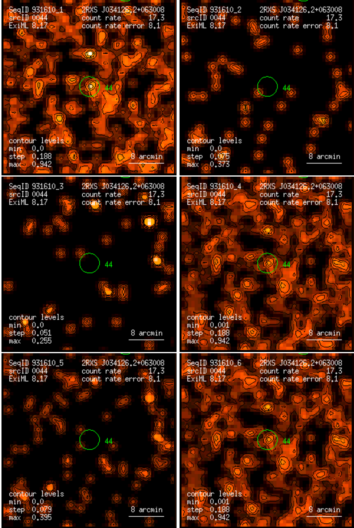
Figure 44: RASS 931610: detection 0044: band rate images, Gaussian filter: (1) PSPC channels 11 – 41, (2) 52 – 90, (3) 91 – 201, (4) 11 – 235, (5) 52 – 201, (6) 11 – 201. Broad band rates in counts/ks. Band rate contour levels in counts/ks/arcmin 2 .
