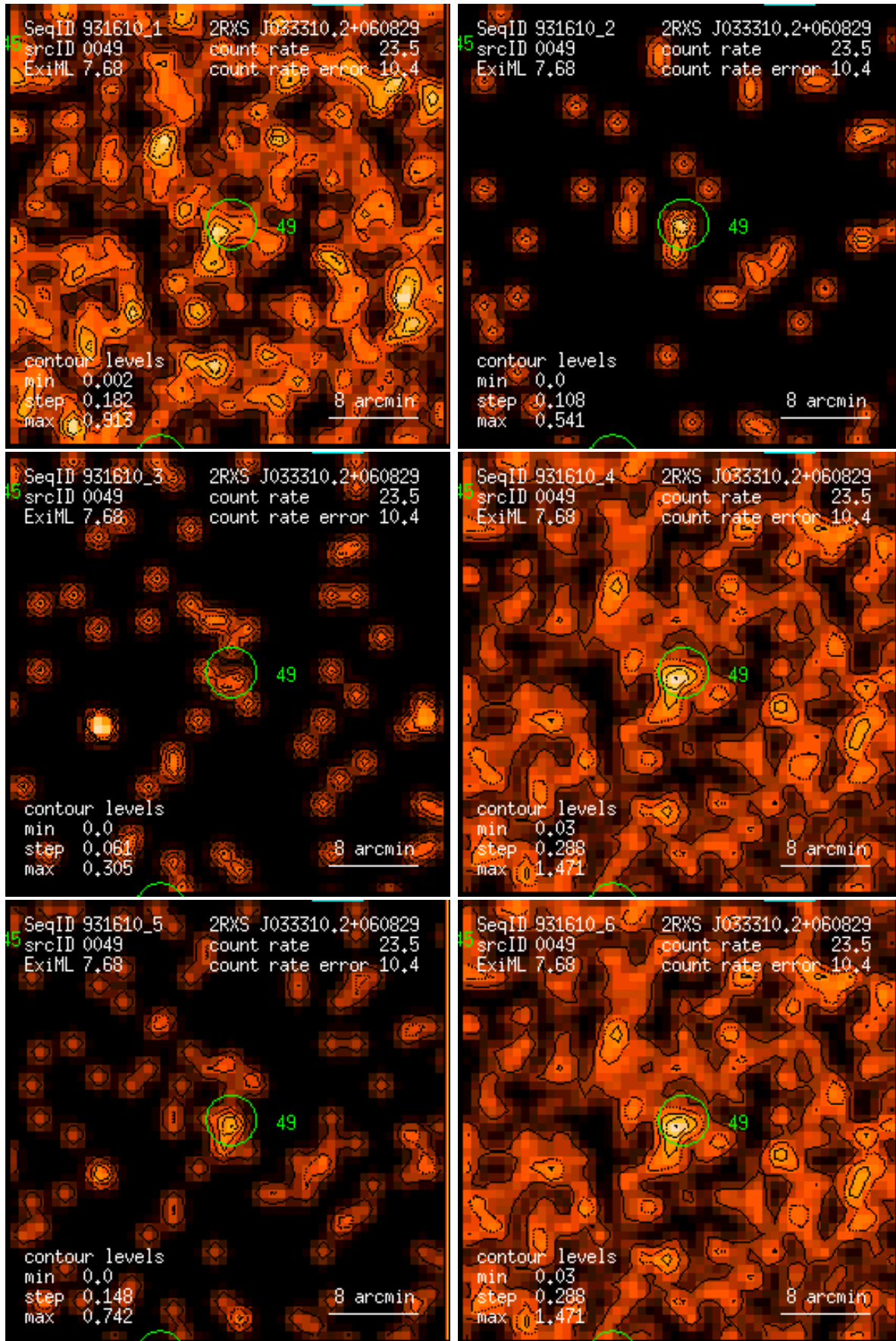
Figure 49: RASS 931610: detection 0049: band rate images, Gaussian filter: (1) PSPC channels 11 – 41, (2) 52 – 90, (3) 91 – 201, (4) 11 – 235, (5) 52 – 201, (6) 11 – 201. Broad band rates in counts/ks. Band rate contour levels in counts/ks/arcmin 2 .
