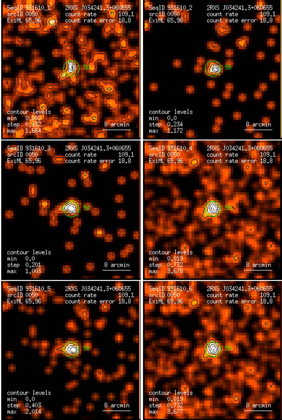
Figure 50: RASS 931610: detection 0050: band rate images, Gaussian filter: (1) PSPC channels 11 – 41, (2) 52 – 90, (3) 91 – 201, (4) 11 – 235, (5) 52 – 201, (6) 11 – 201. Broad band rates in counts/ks. Band rate contour levels in counts/ks/arcmin 2 .
