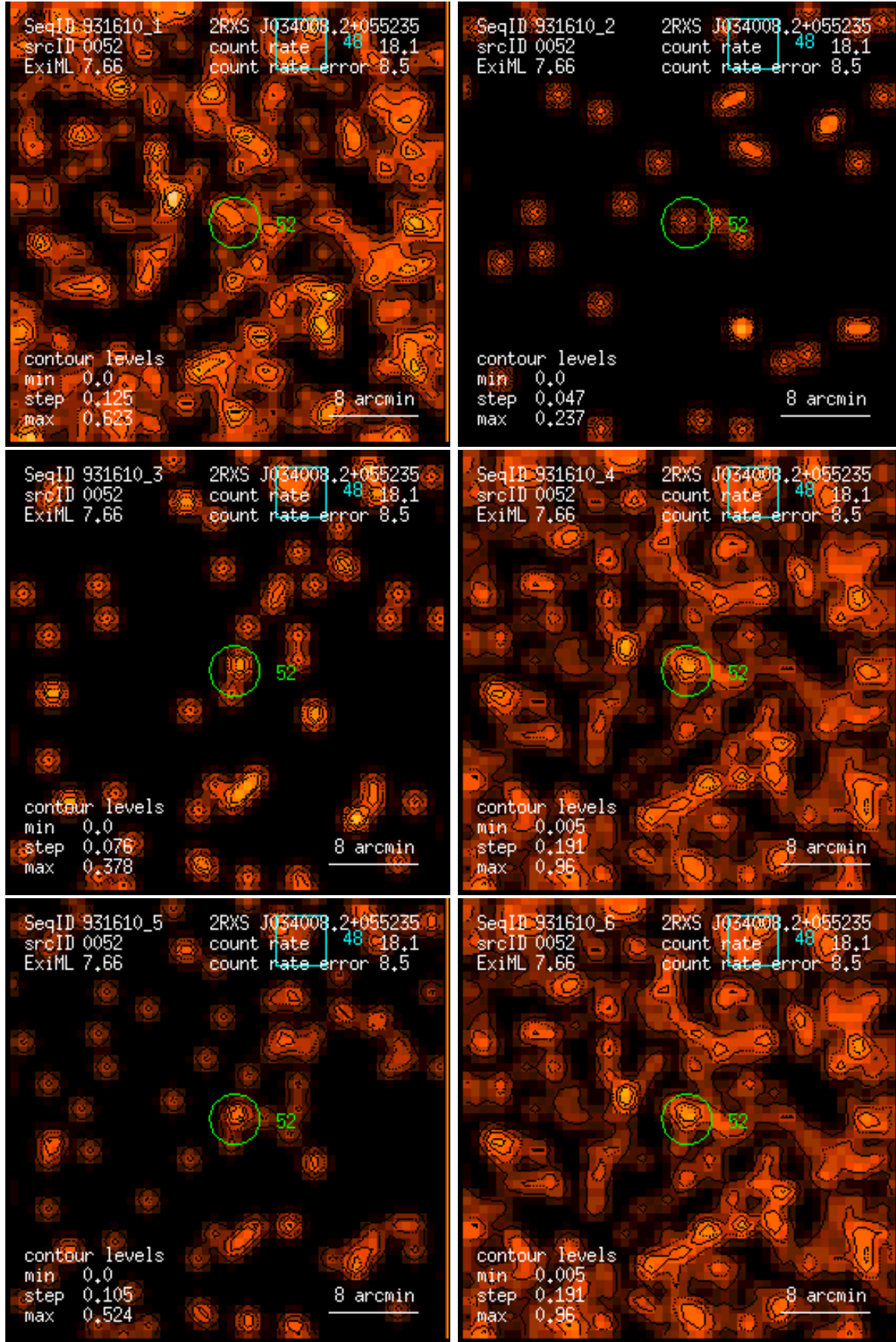
Figure 52: RASS 931610: detection 0052: band rate images, Gaussian filter: (1) PSPC channels 11 – 41, (2) 52 – 90, (3) 91 – 201, (4) 11 – 235, (5) 52 – 201, (6) 11 – 201. Broad band rates in counts/ks. Band rate contour levels in counts/ks/arcmin 2 .
