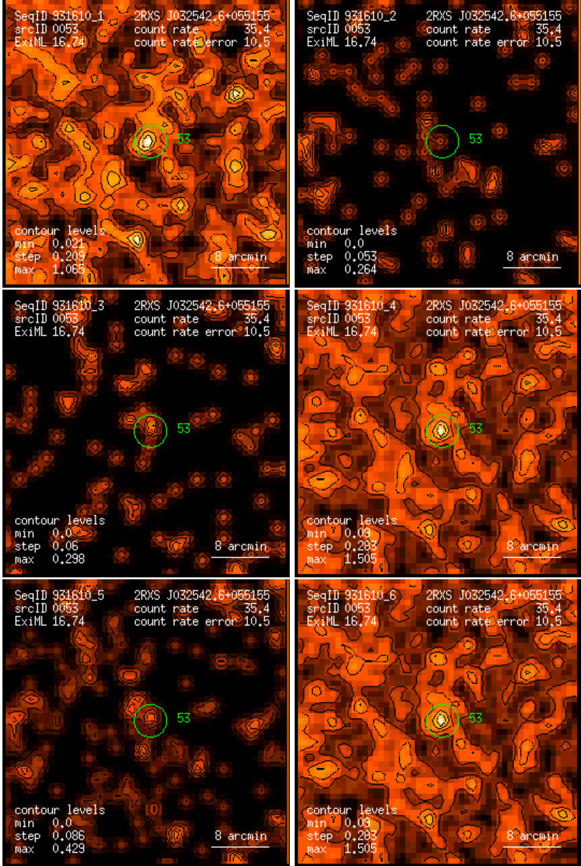
Figure 53: RASS 931610: detection 0053: band rate images, Gaussian filter: (1) PSPC channels 11 – 41, (2) 52 – 90, (3) 91 – 201, (4) 11 – 235, (5) 52 – 201, (6) 11 – 201. Broad band rates in counts/ks. Band rate contour levels in counts/ks/arcmin 2 .
