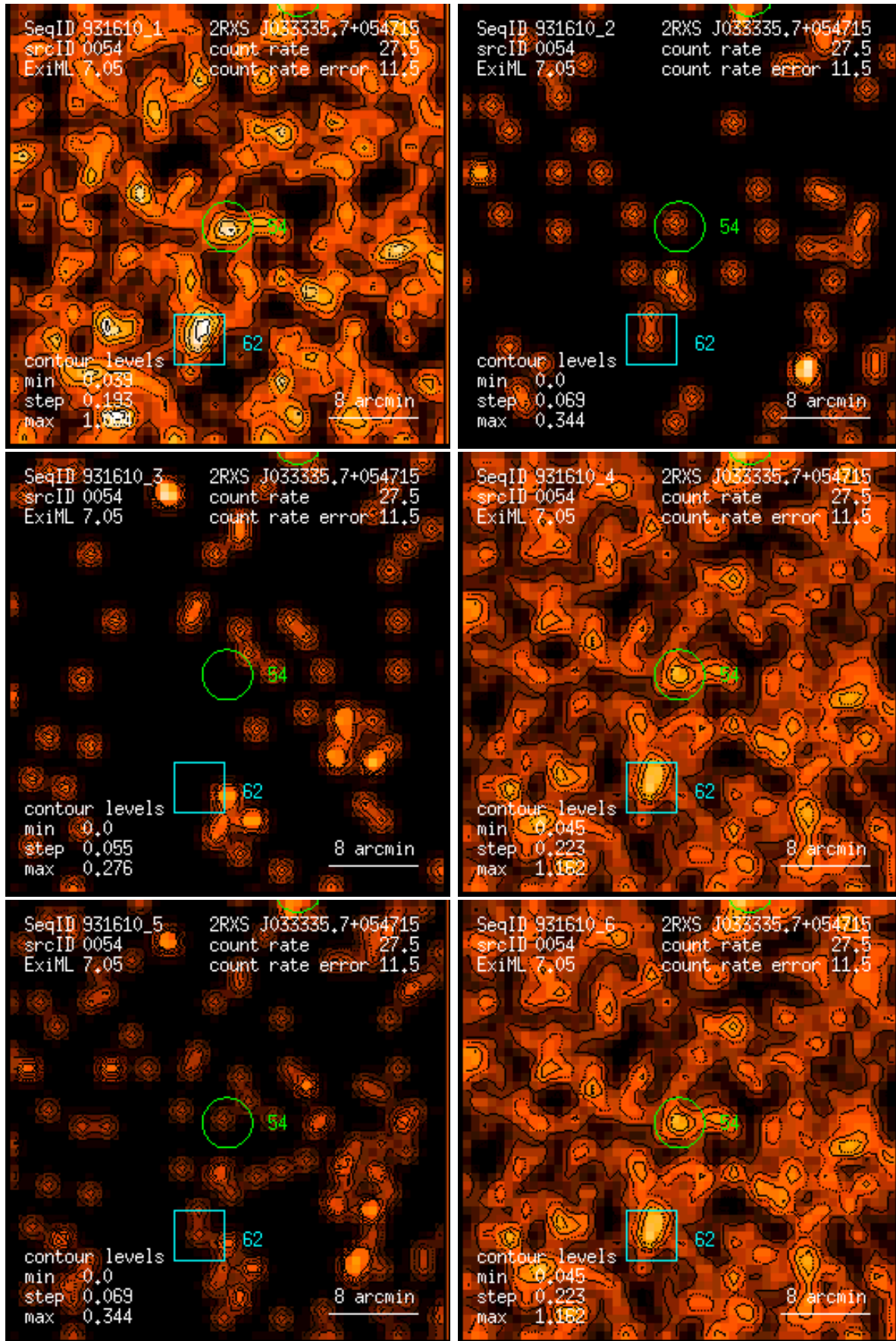
Figure 54: RASS 931610: detection 0054: band rate images, Gaussian filter: (1) PSPC channels 11 – 41, (2) 52 – 90, (3) 91 – 201, (4) 11 – 235, (5) 52 – 201, (6) 11 – 201. Broad band rates in counts/ks. Band rate contour levels in counts/ks/arcmin 2 .
