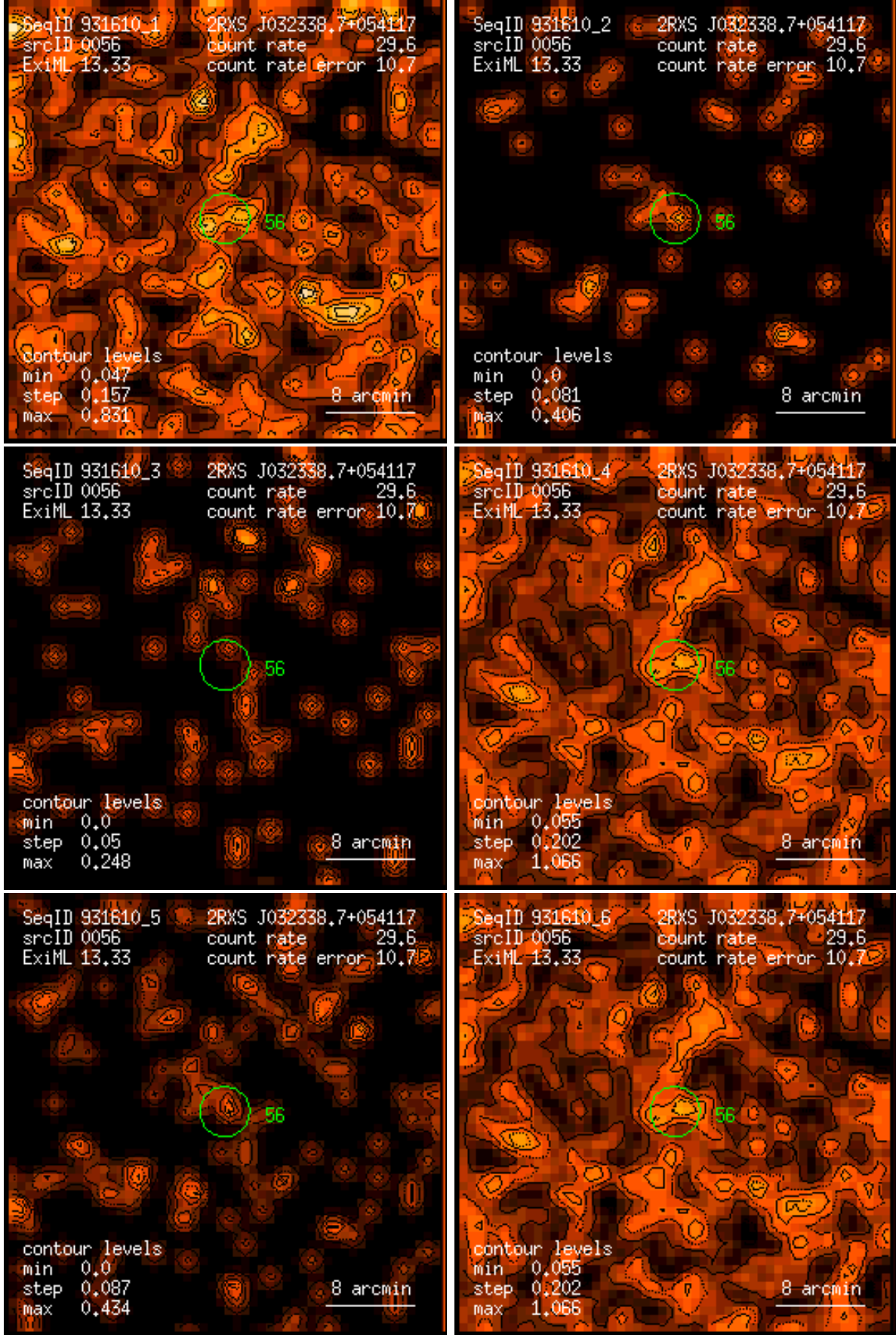
Figure 56: RASS 931610: detection 0056: band rate images, Gaussian filter: (1) PSPC channels 11 – 41, (2) 52 – 90, (3) 91 – 201, (4) 11 – 235, (5) 52 – 201, (6) 11 – 201. Broad band rates in counts/ks. Band rate contour levels in counts/ks/arcmin 2 .
