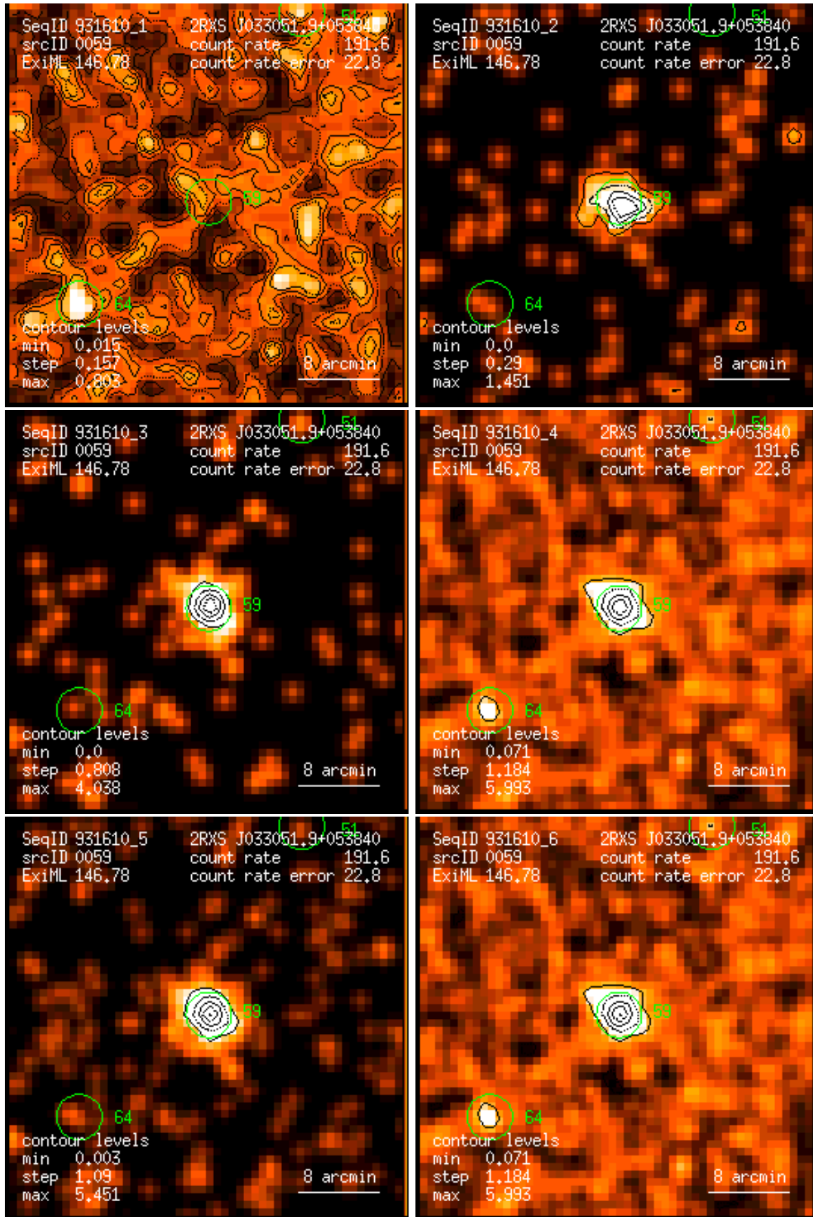
Figure 59: RASS 931610: detection 0059: band rate images, Gaussian filter: (1) PSPC channels 11 – 41, (2) 52 – 90, (3) 91 – 201, (4) 11 – 235, (5) 52 – 201, (6) 11 – 201. Broad band rates in counts/ks. Band rate contour levels in counts/ks/arcmin 2 .
