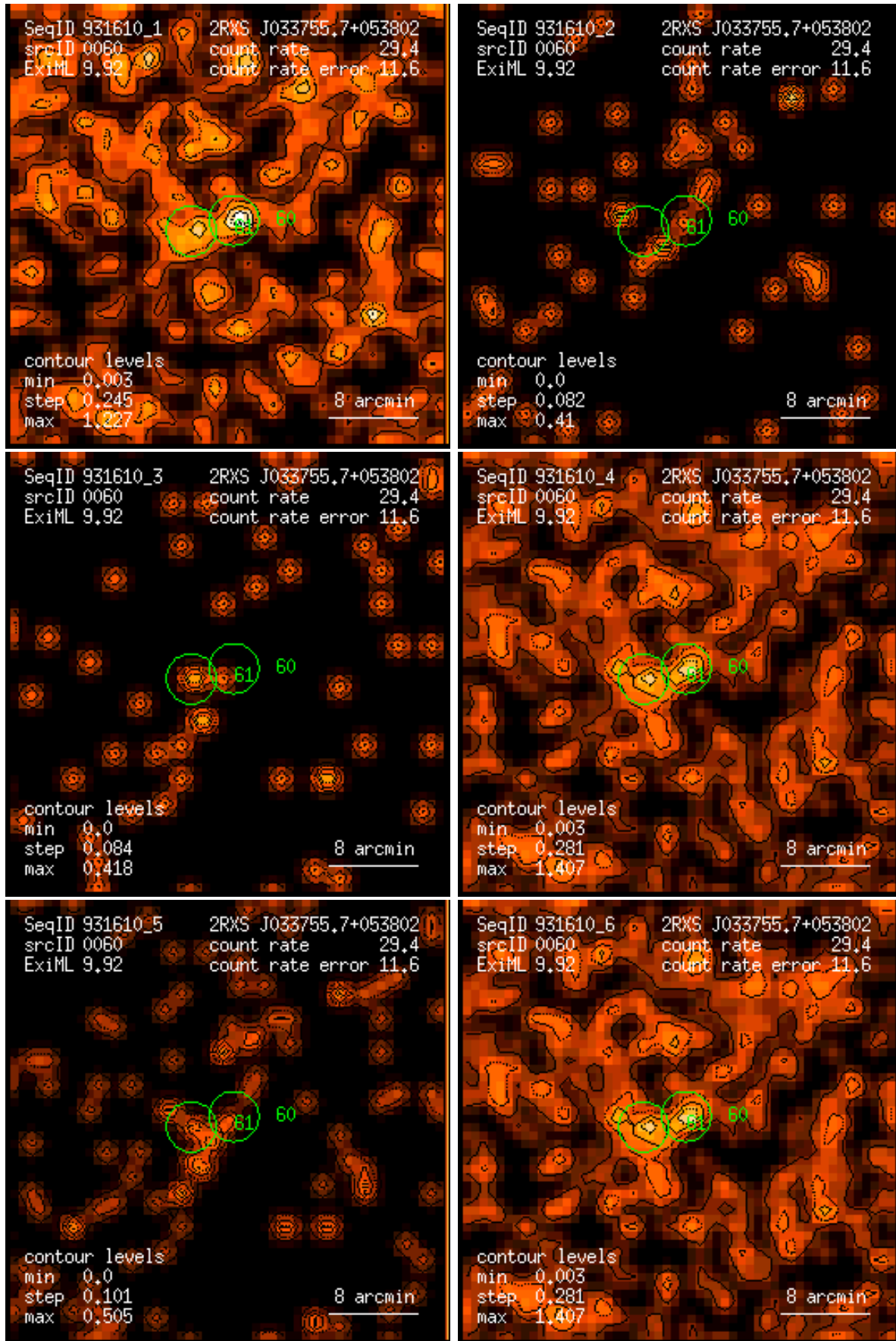
Figure 60: RASS 931610: detection 0060: band rate images, Gaussian filter: (1) PSPP channels 11 – 41, (2) 52 – 90, (3) 91 – 201, (4) 11 – 235, (5) 52 – 201, (6) 11 – 201. Broad band rates in counts/ks. Band rate contour levels in counts/ks/arcmin 2 .
