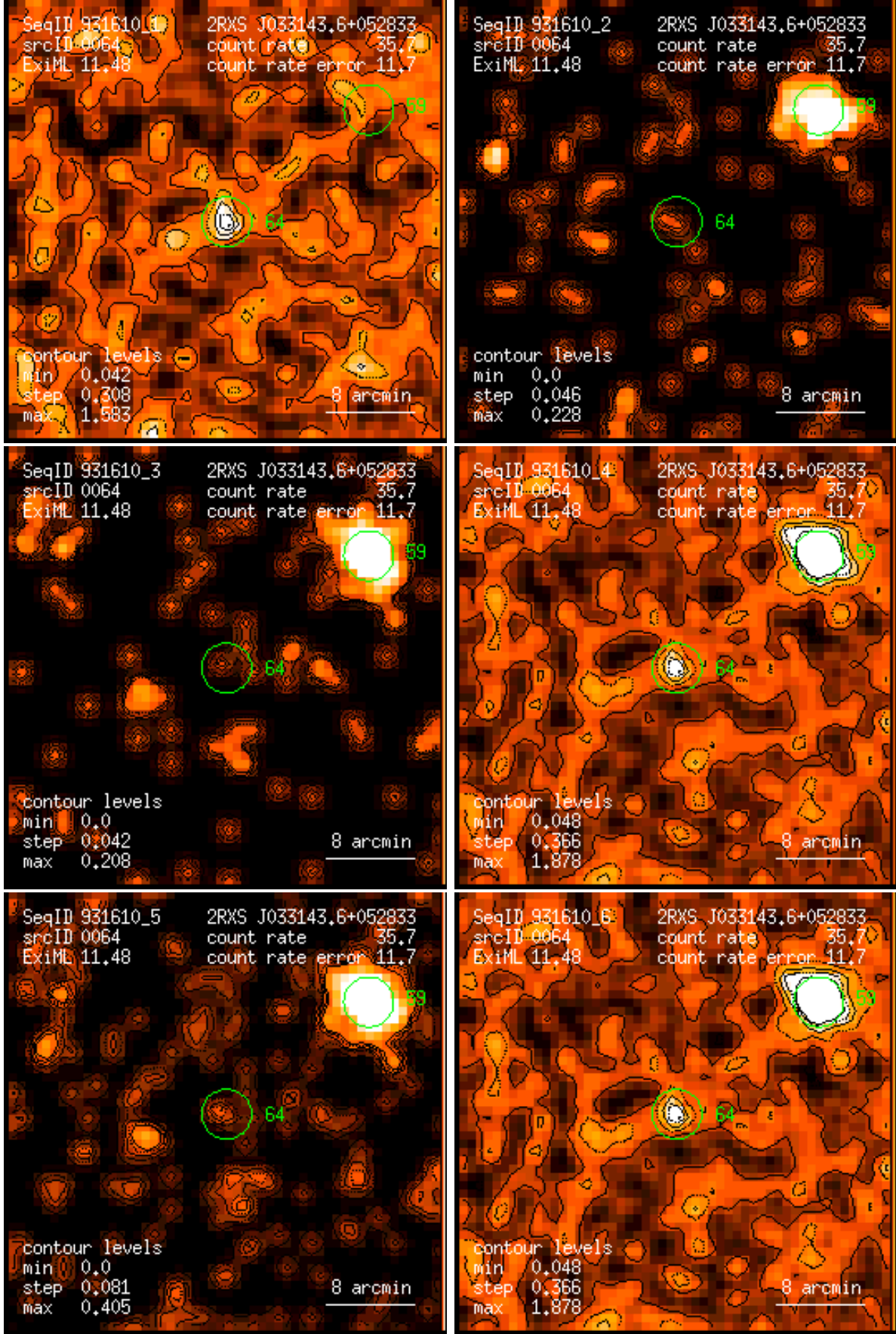
Figure 64: RASS 931610: detection 0064: band rate images, Gaussian filter: (1) PSPC channels 11 – 41, (2) 52 – 90, (3) 91 – 201, (4) 11 – 235, (5) 52 – 201, (6) 11 – 201. Broad band rates in counts/ks. Band rate contour levels in counts/ks/arcmin 2 .
