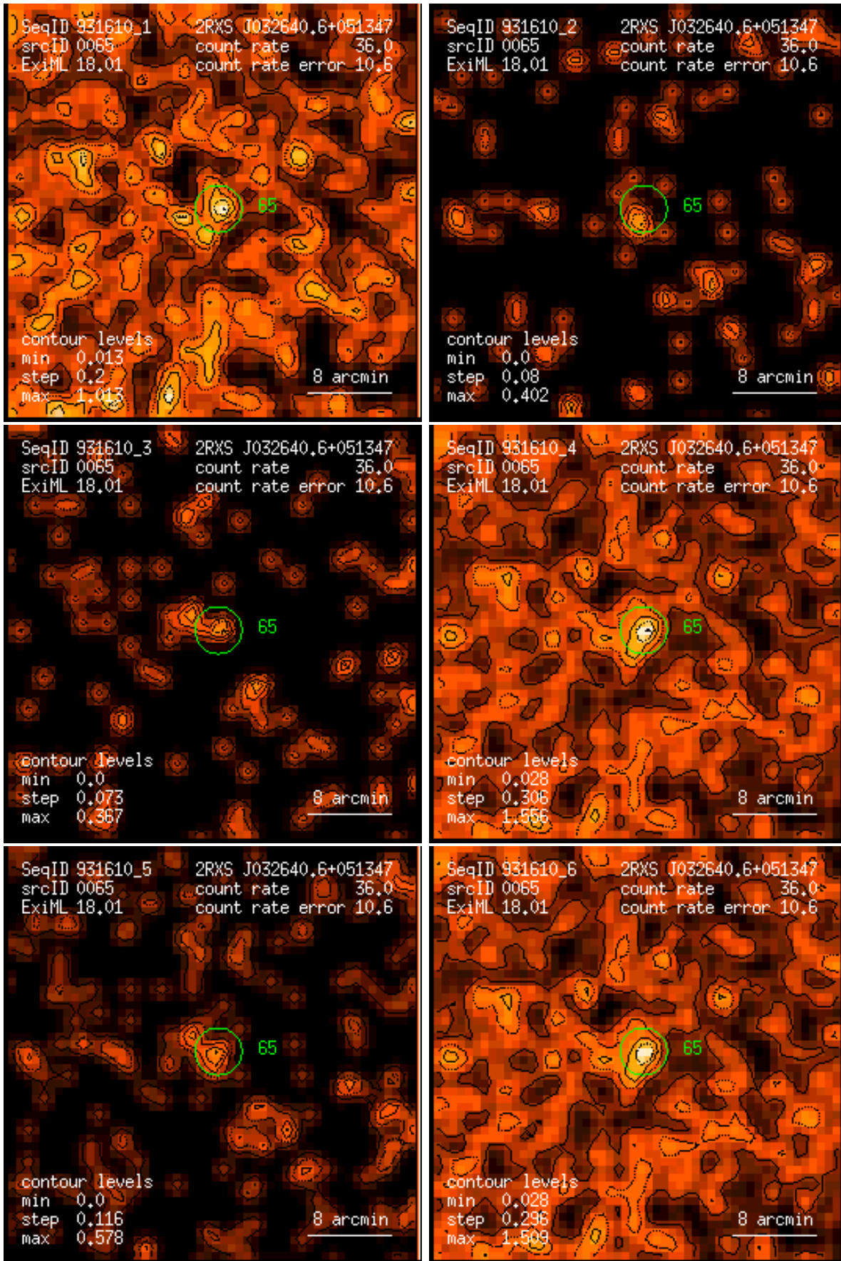
Figure 65: RASS 931610: detection 0065: band rate images, Gaussian filter: (1) PSPC channels 11 – 41, (2) 52 – 90, (3) 91 – 201, (4) 11 – 235, (5) 52 – 201, (6) 11 – 201. Broad band rates in counts/ks. Band rate contour levels in counts/ks/arcmin 2 .
