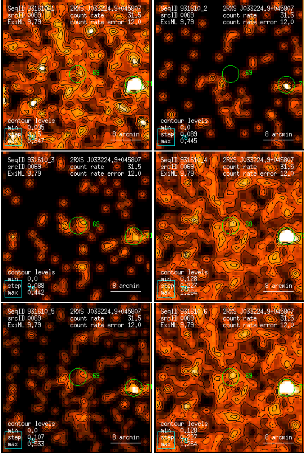
Figure 69: RASS 931610: detection 0069: band rate images, Gaussian filter: (1) PSPC channels 11 – 41, (2) 52 – 90, (3) 91 – 201, (4) 11 – 235, (5) 52 – 201, (6) 11 – 201. Broad band rates in counts/ks. Band rate contour levels in counts/ks/arcmin 2 .
