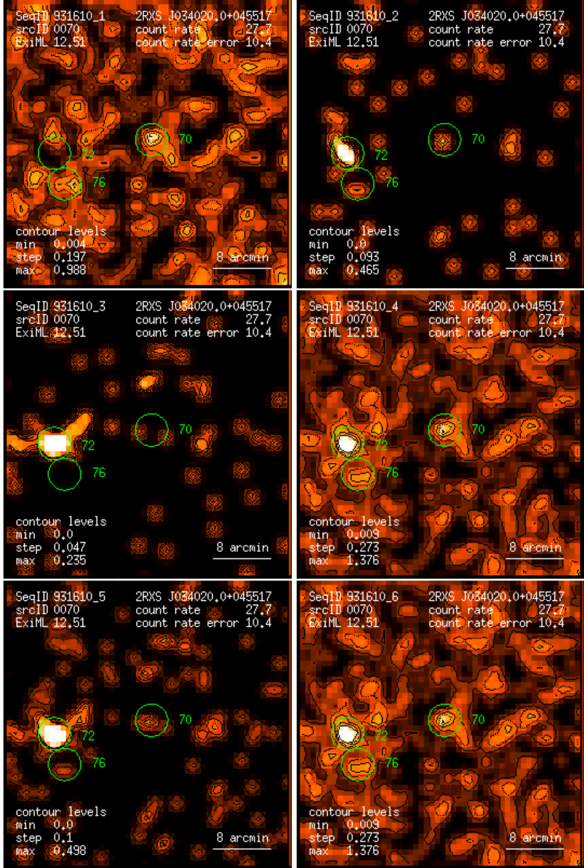
Figure 70: RASS 931610: detection 0070: band rate images, Gaussian filter: (1) PSPC channels 11 – 41, (2) 52 – 90, (3) 91 – 201, (4) 11 – 235, (5) 52 – 201, (6) 11 – 201. Broad band rates in counts/ks. Band rate contour levels in counts/ks/arcmin 2 .
