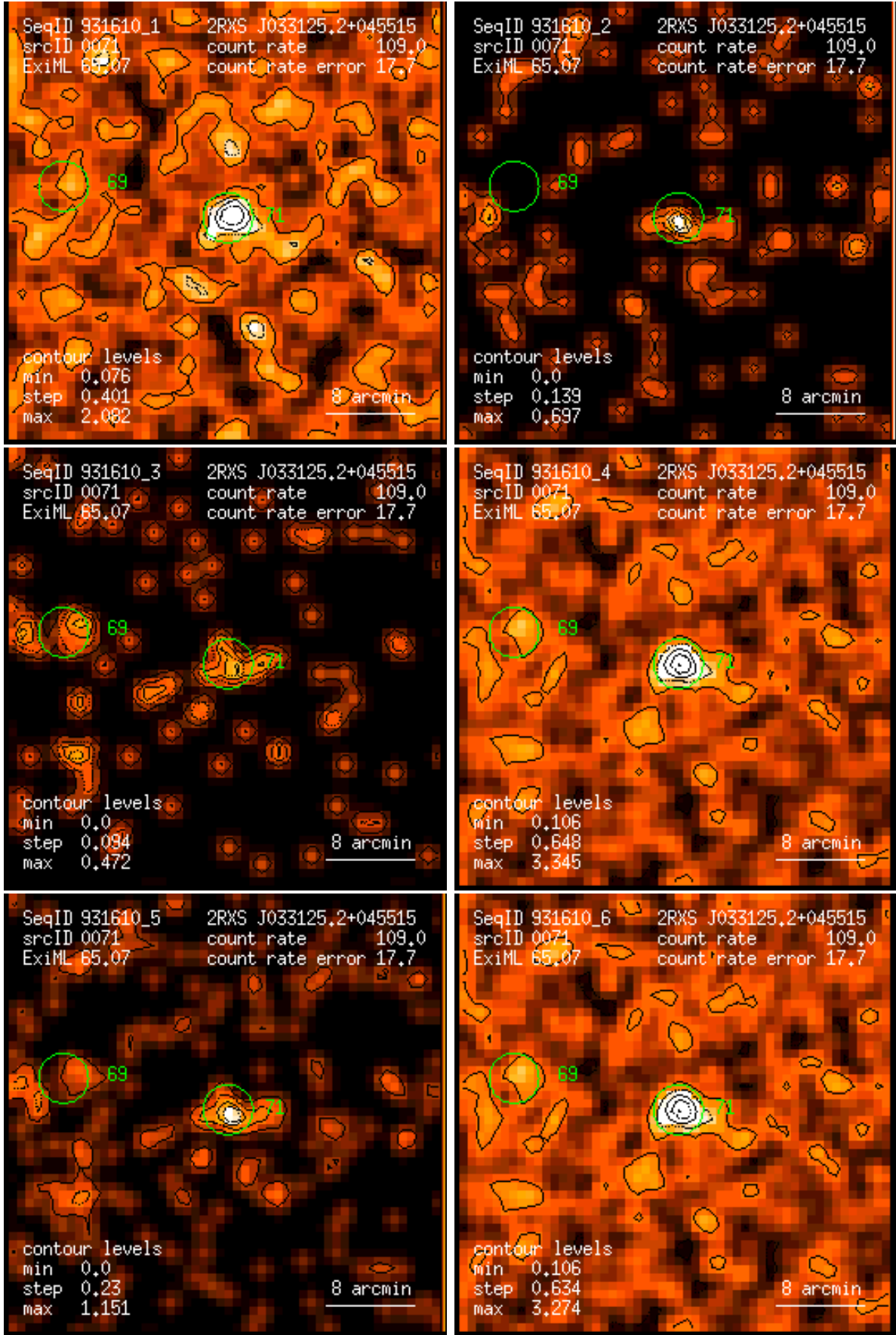
Figure 71: RASS 931610: detection 0071: band rate images, Gaussian filter: (1) PSPC channels 11 – 41, (2) 52 – 90, (3) 91 – 201, (4) 11 – 235, (5) 52 – 201, (6) 11 – 201. Broad band rates in counts/ks. Band rate contour levels in counts/ks/arcmin 2 .
