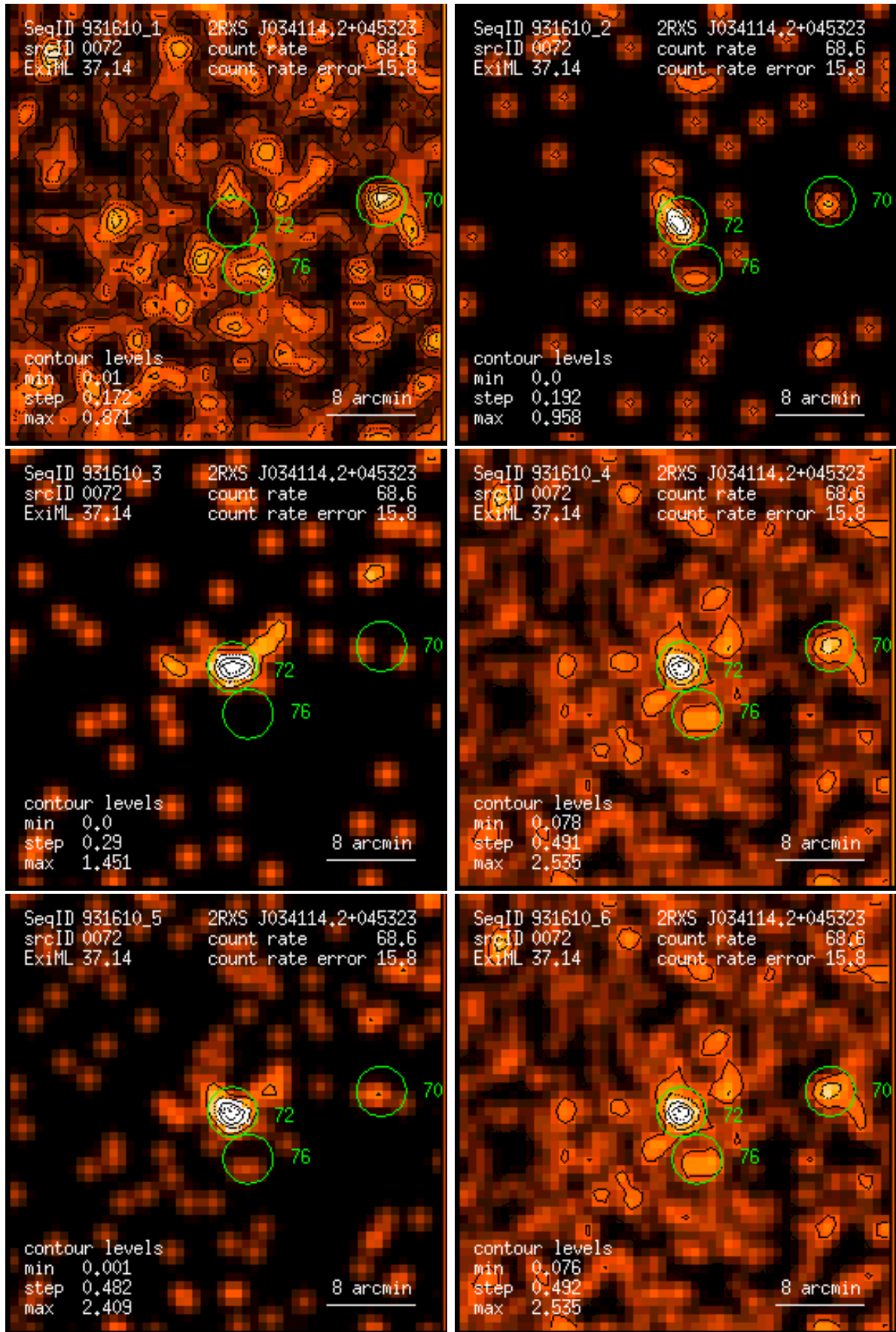
Figure 72: RASS 931610: detection 0072: band rate images, Gaussian filter: (1) PSPC channels 11 – 41, (2) 52 – 90, (3) 91 – 201, (4) 11 – 235, (5) 52 – 201, (6) 11 – 201. Broad band rates in counts/ks. Band rate contour levels in counts/ks/arcmin 2 .
