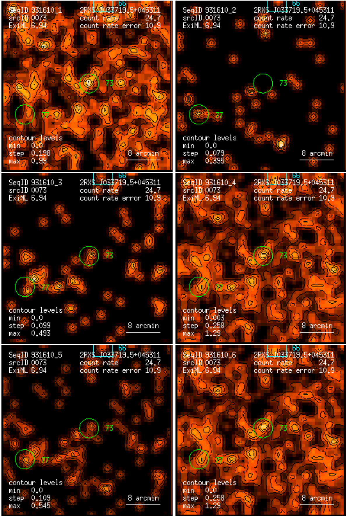
Figure 73: RASS 931610: detection 0073: band rate images, Gaussian filter: (1) PSPC channels 11 – 41, (2) 52 – 90, (3) 91 – 201, (4) 11 – 235, (5) 52 – 201, (6) 11 – 201. Broad band rates in counts/ks. Band rate contour levels in counts/ks/arcmin 2 .
