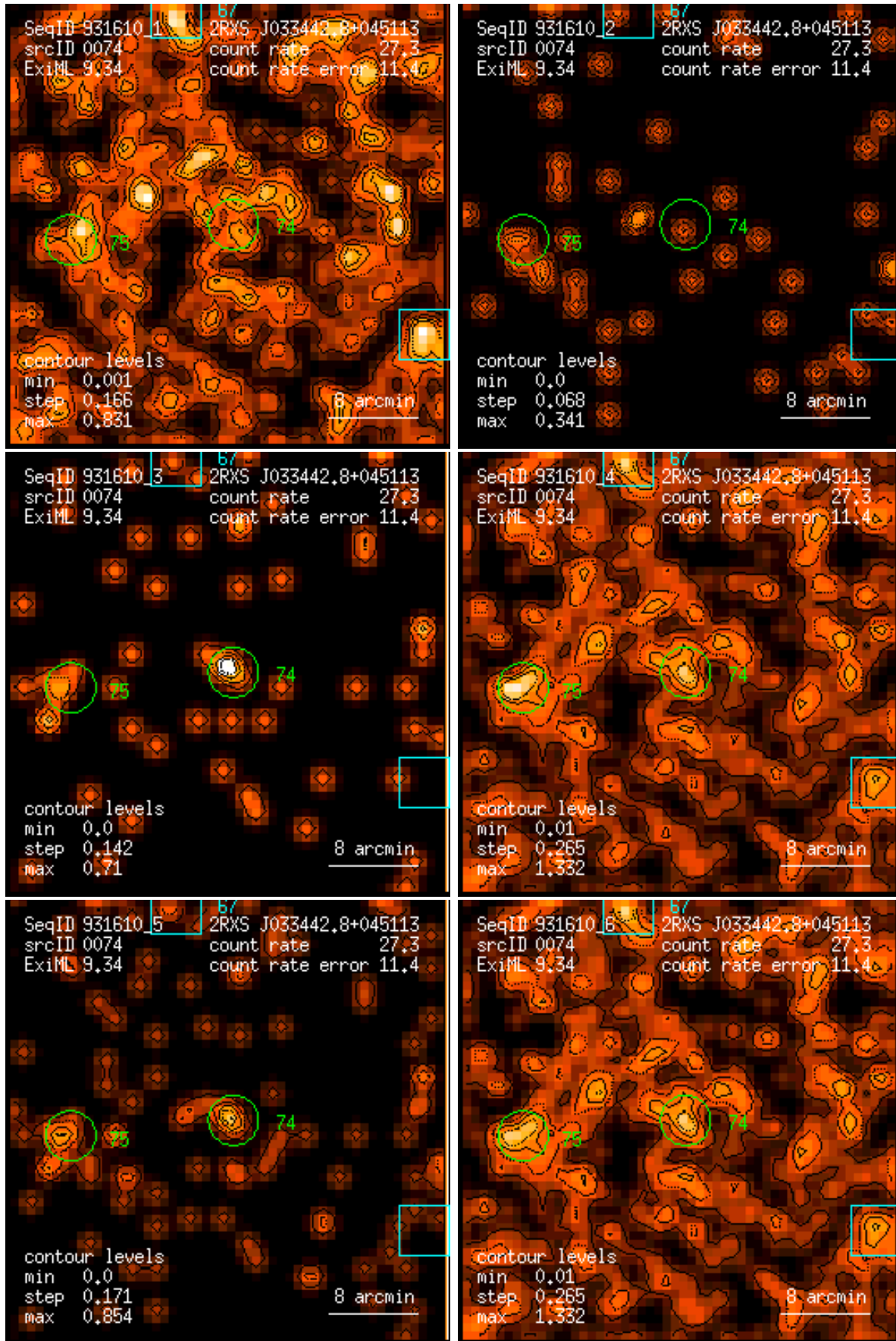
Figure 74: RASS 931610: detection 0074: band rate images, Gaussian filter: (1) PSPC channels 11 – 41, (2) 52 – 90, (3) 91 – 201, (4) 11 – 235, (5) 52 – 201, (6) 11 – 201. Broad band rates in counts/ks. Band rate contour levels in counts/ks/arcmin 2 .
