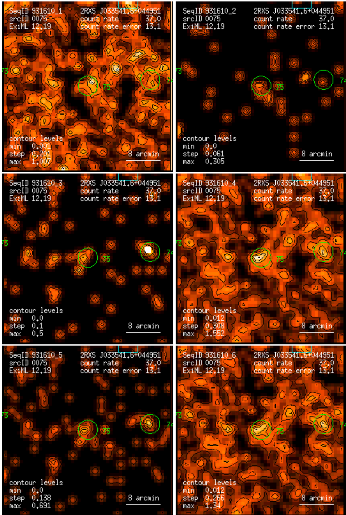
Figure 75: RASS 931610: detection 0075: band rate images, Gaussian filter: (1) PSPC channels 11 – 41, (2) 52 – 90, (3) 91 – 201, (4) 11 – 235, (5) 52 – 201, (6) 11 – 201. Broad band rates in counts/ks. Band rate contour levels in counts/ks/arcmin 2 .
