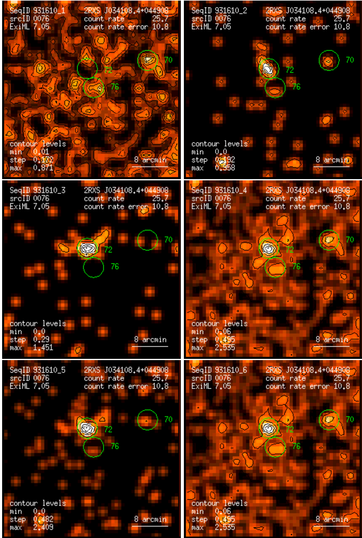
Figure 76: RASS 931610: detection 0076: band rate images, Gaussian filter: (1) PSPC channels 11 – 41, (2) 52 – 90, (3) 91 – 201, (4) 11 – 235, (5) 52 – 201, (6) 11 – 201. Broad band rates in counts/ks. Band rate contour levels in counts/ks/arcmin 2 .
