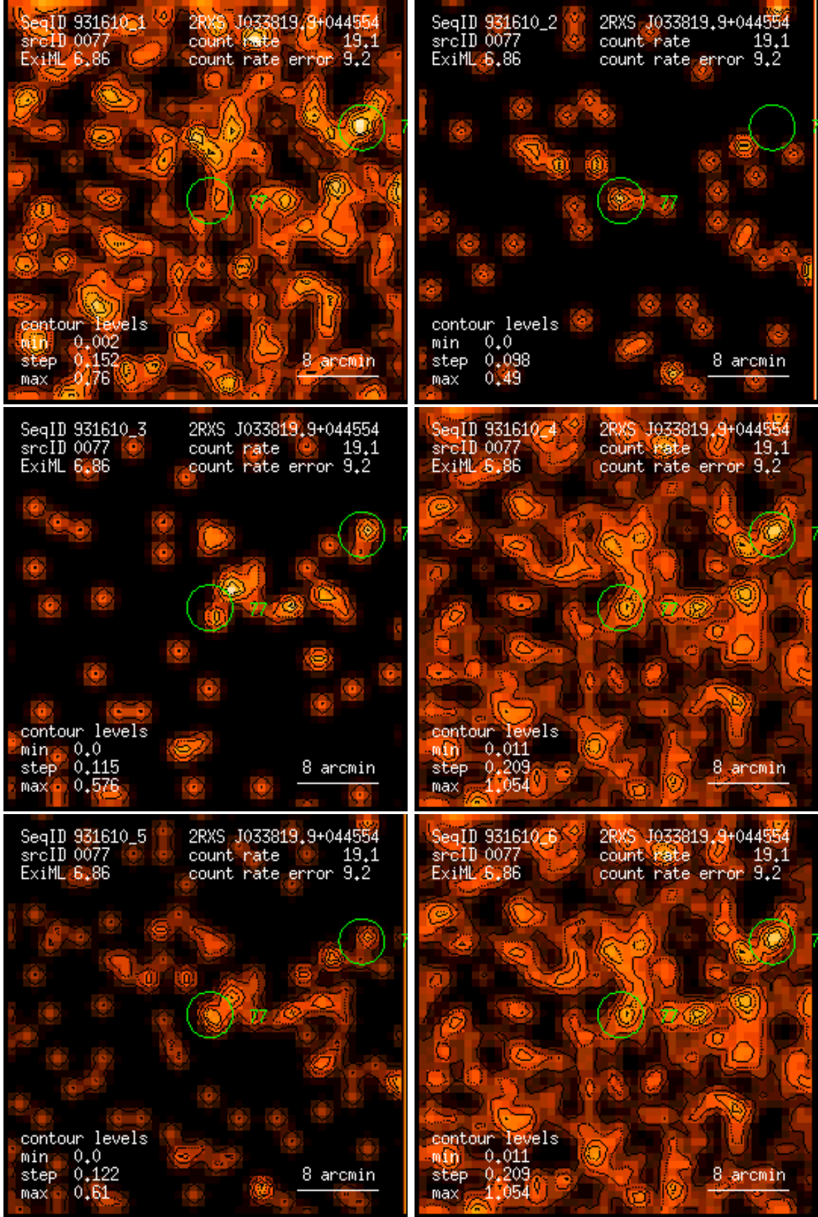
Figure 77: RASS 931610: detection 0077: band rate images, Gaussian filter: (1) PSPC channels 11 – 41, (2) 52 – 90, (3) 91 – 201, (4) 11 – 235, (5) 52 – 201, (6) 11 – 201. Broad band rates in counts/ks. Band rate contour levels in counts/ks/arcmin 2 .
