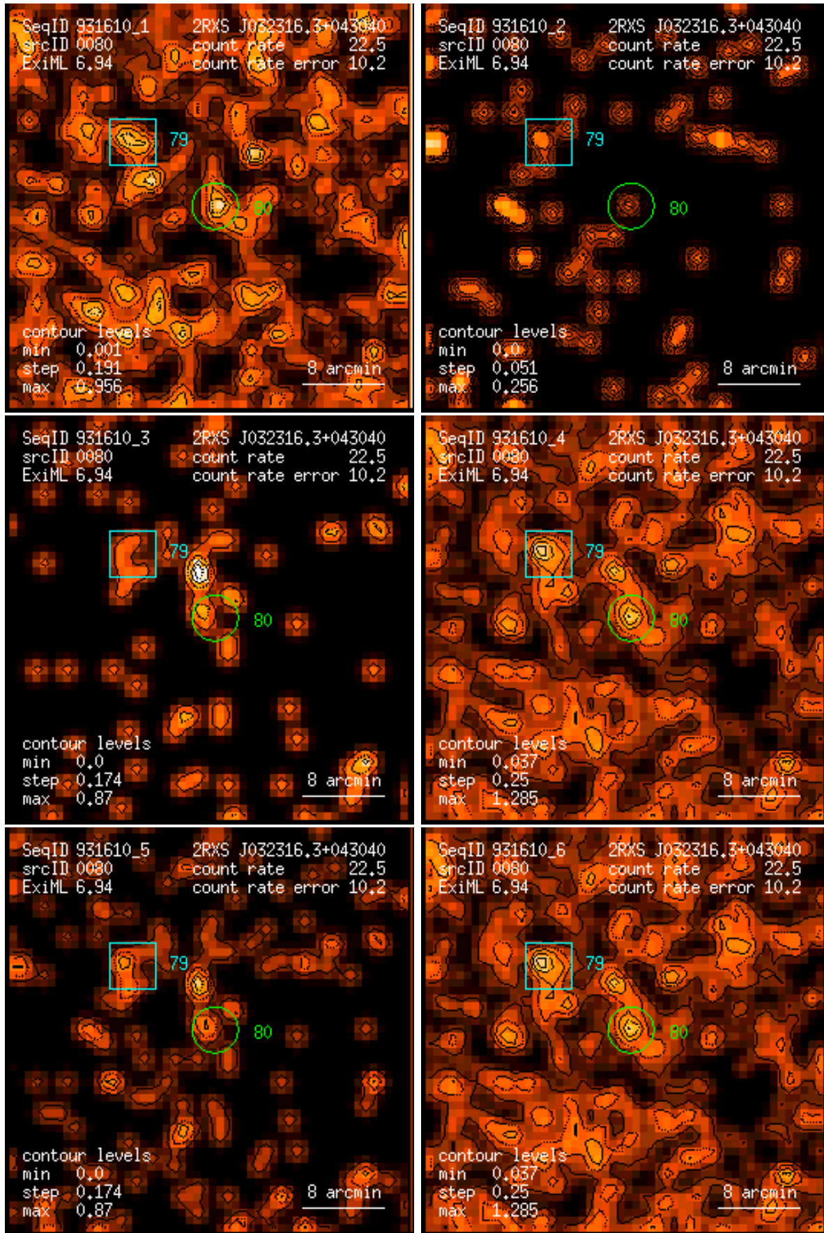
Figure 80: RASS 931610: detection 0080: band rate images, Gaussian filter: (1) PSPC channels 11 – 41, (2) 52 – 90, (3) 91 – 201, (4) 11 – 235, (5) 52 – 201, (6) 11 – 201. Broad band rates in counts/ks. Band rate contour levels in counts/ks/arcmin 2 .
