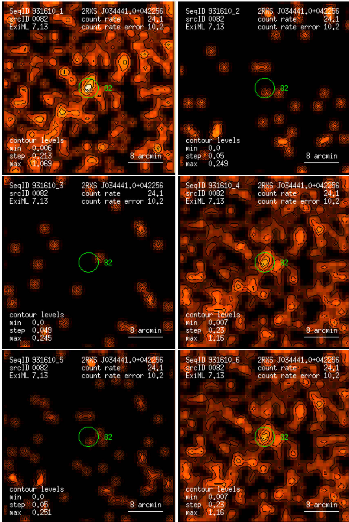
Figure 82: RASS 931610: detection 0082: band rate images, Gaussian filter: (1) PSPC channels 11 – 41, (2) 52 – 90, (3) 91 – 201, (4) 11 – 235, (5) 52 – 201, (6) 11 – 201. Broad band rates in counts/ks. Band rate contour levels in counts/ks/arcmin 2 .
