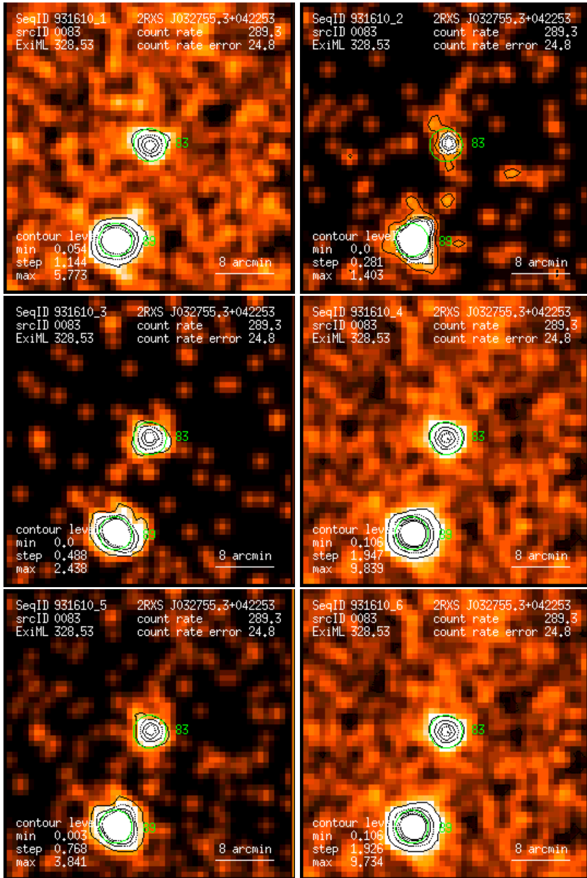
Figure 83: RASS 931610: detection 0083: band rate images, Gaussian filter: (1) PSPC channels 11 – 41, (2) 52 – 90, (3) 91 – 201, (4) 11 – 235, (5) 52 – 201, (6) 11 – 201. Broad band rates in counts/ks. Band rate contour levels in counts/ks/arcmin 2 .
