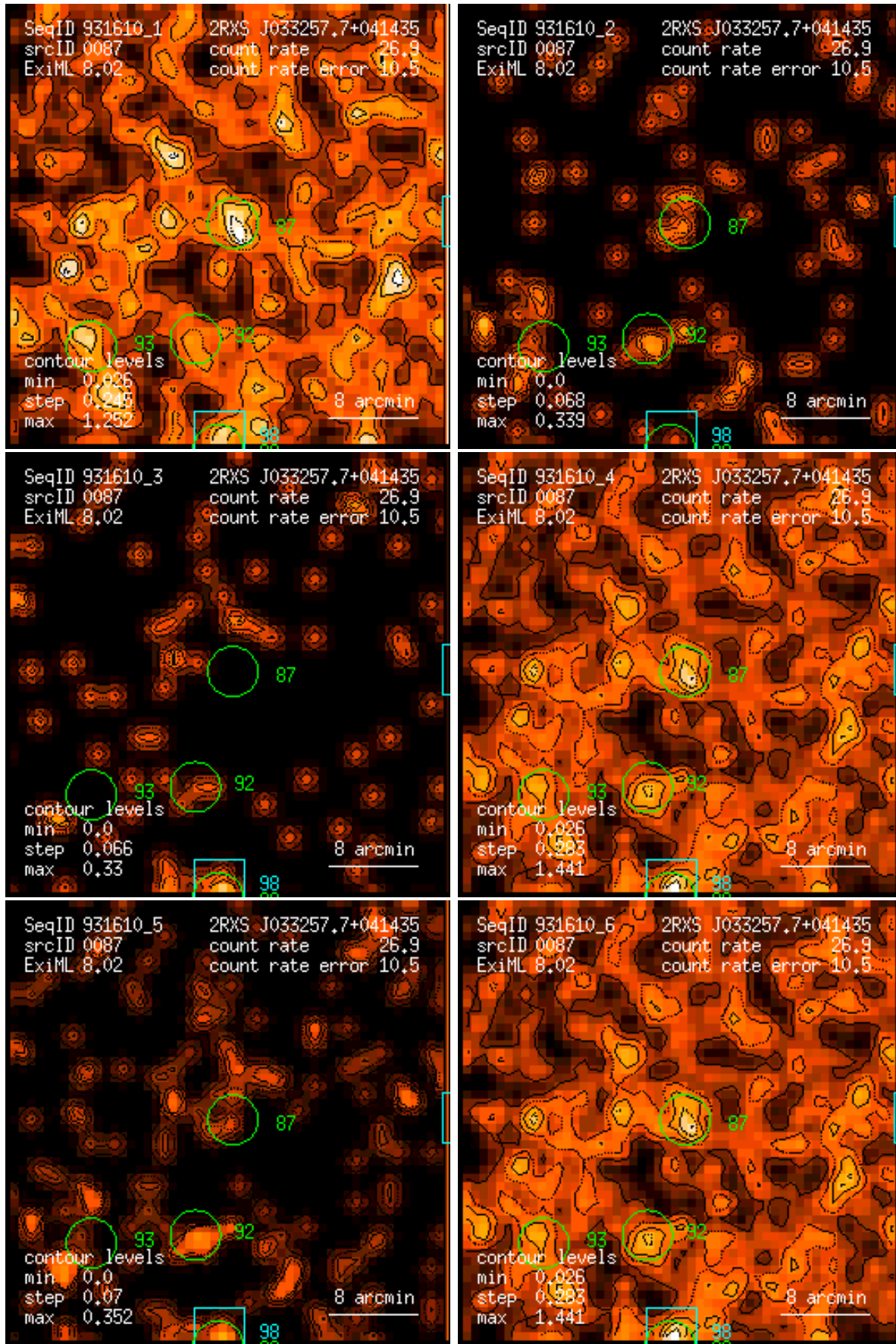
Figure 87: RASS 931610: detection 0087: band rate images, Gaussian filter: (1) PSPC channels 11 – 41, (2) 52 – 90, (3) 91 – 201, (4) 11 – 235, (5) 52 – 201, (6) 11 – 201. Broad band rates in counts/ks. Band rate contour levels in counts/ks/arcmin 2 .
